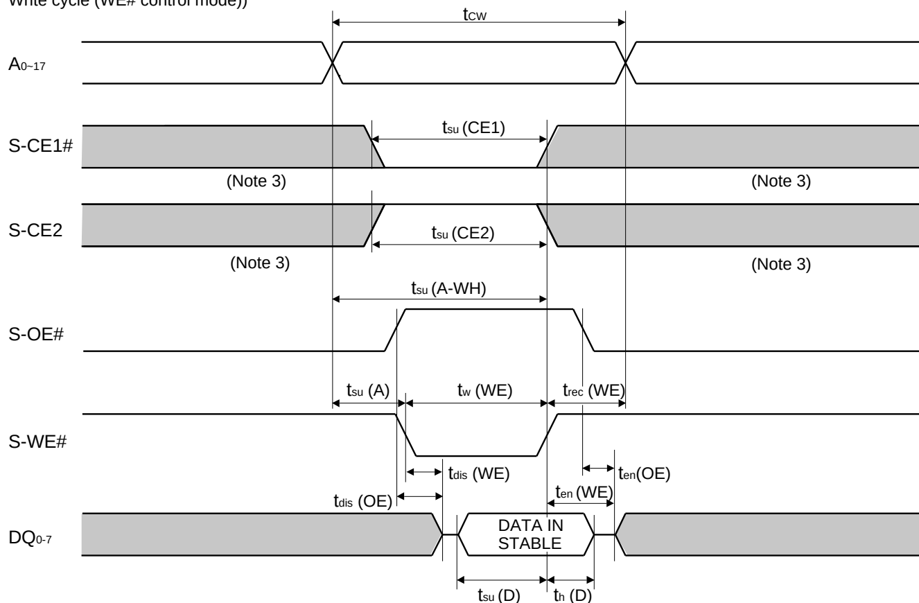
Write cycle (WE# control mode)
