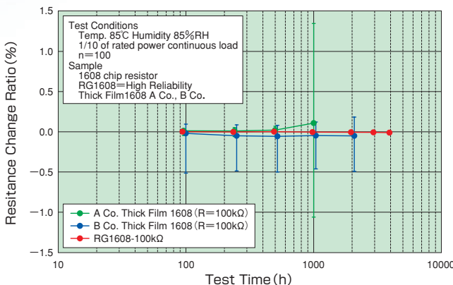
●Temperature Humidity Bias (THB) 85°C 85%
