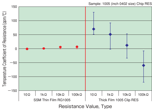
●Temperature Coefficient of Resistance -Thin Film (Susumu) vs Thick Film (Competitor)-
