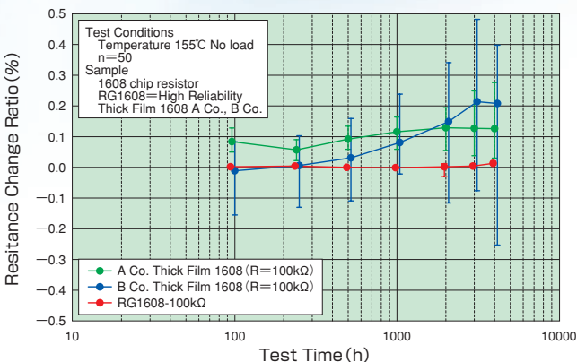
●High Temperature Storage Test 155°C
