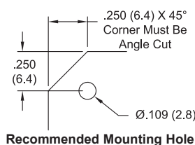
Recommended Mounting Hole
