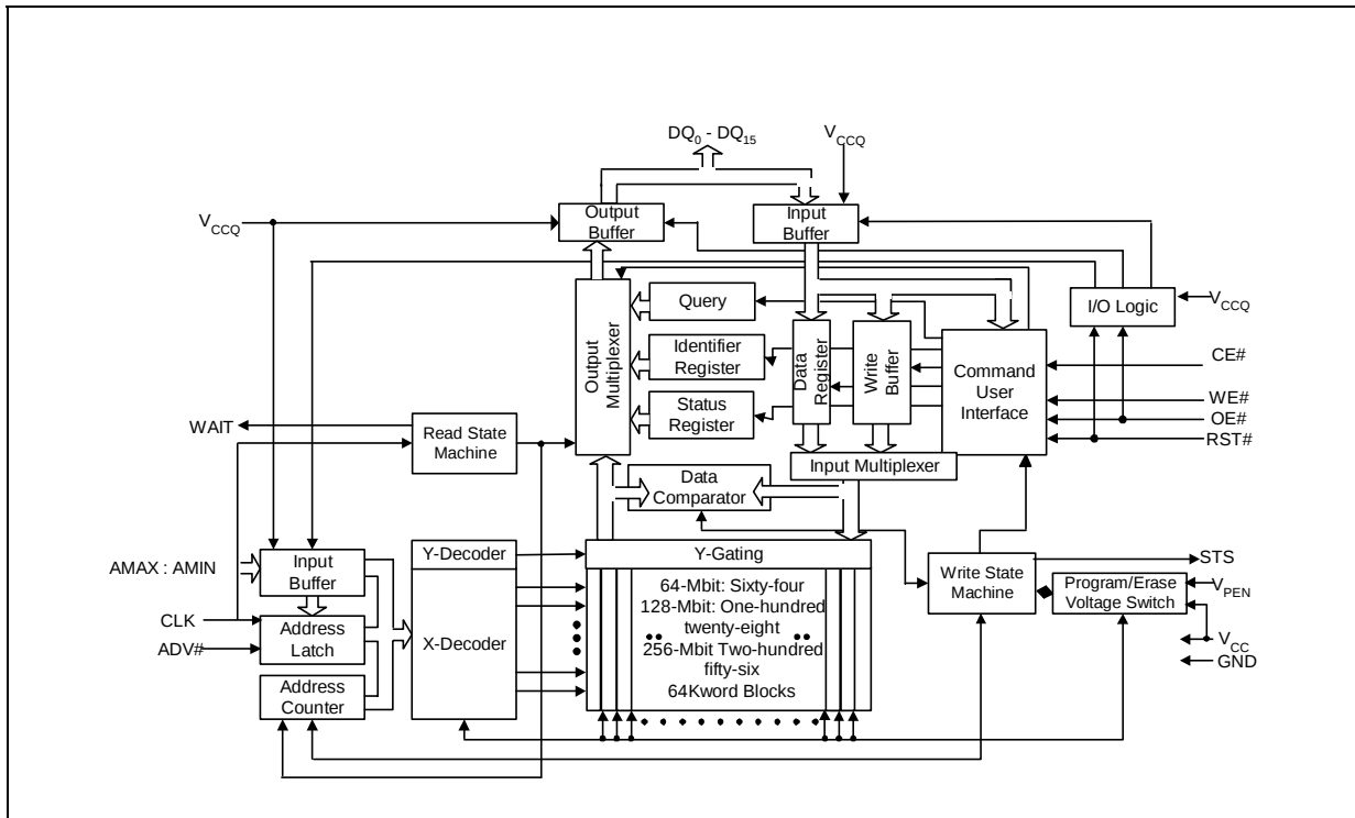
Figure 4. K3/K18 Device Memory Block Diagram
