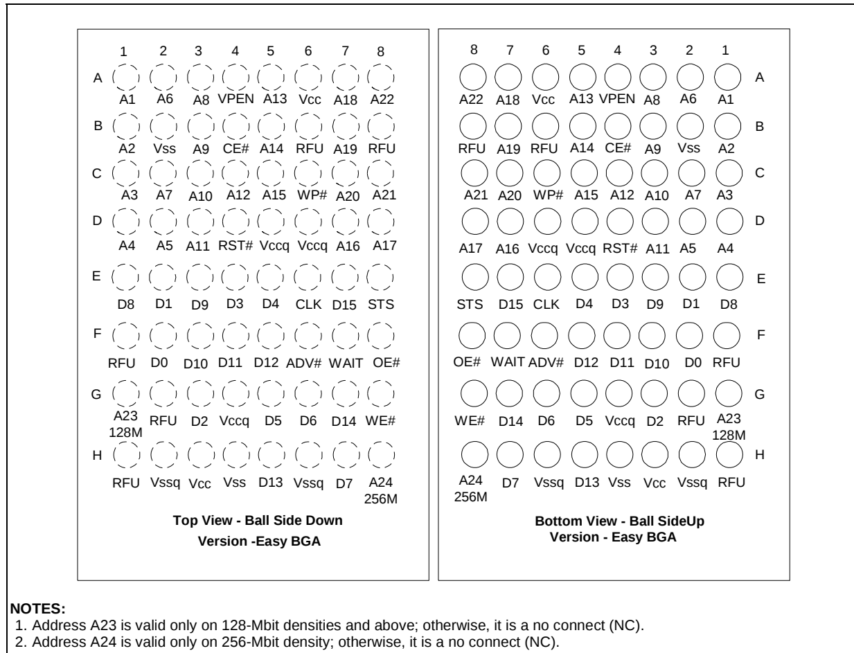
Figure 1. 64-Ball Easy BGA Package, 1.0 mm Ball Pitch
