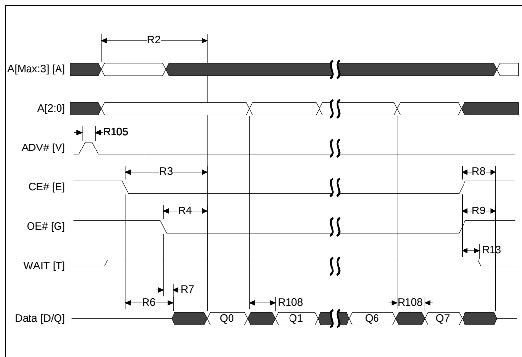
Figure 12. Page Mode Read Waveform
