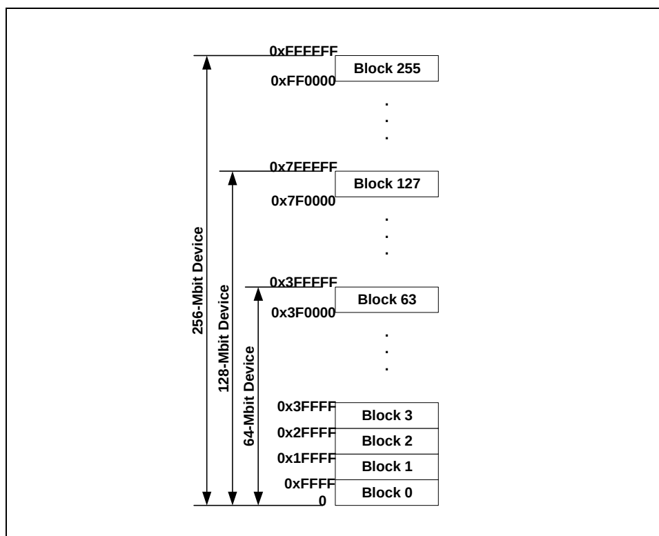
Figure 5. K3/K18 Device Memory Map
