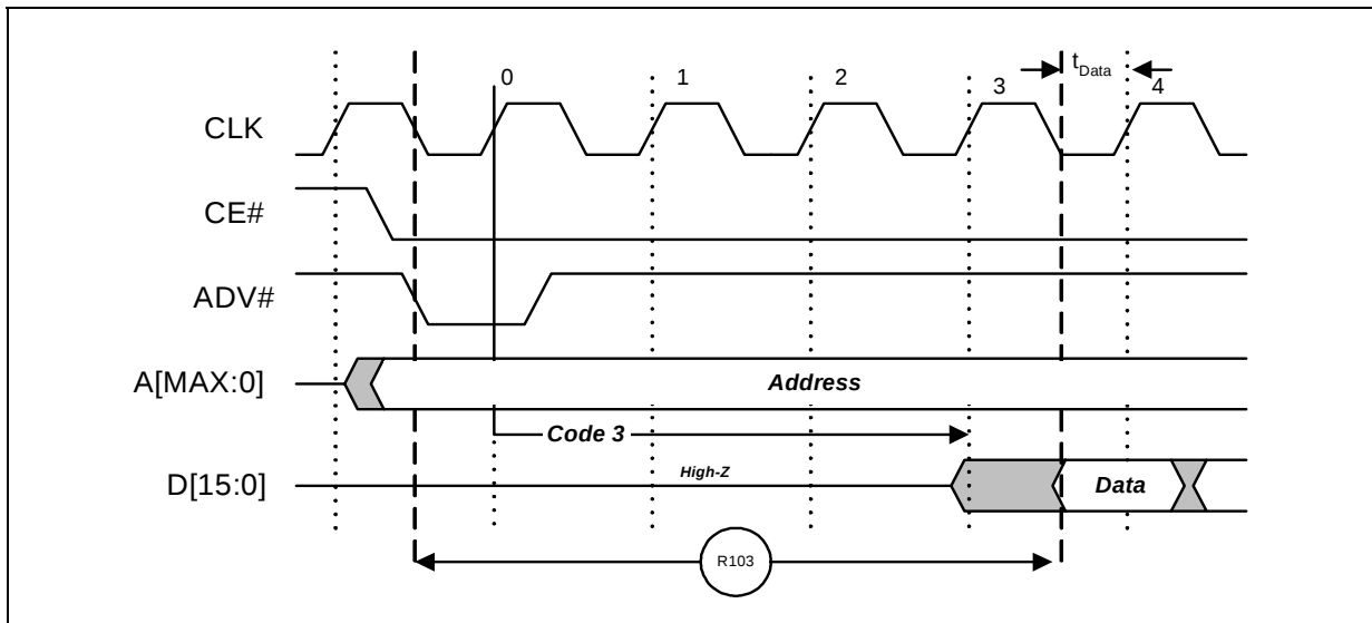
Figure 7. Example Latency Count Setting
