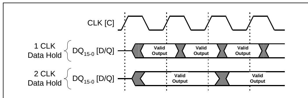
Figure 8. Data Hold Timing
