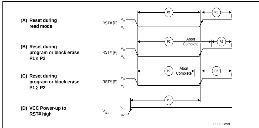
Figure 19. Reset Operation Waveforms
