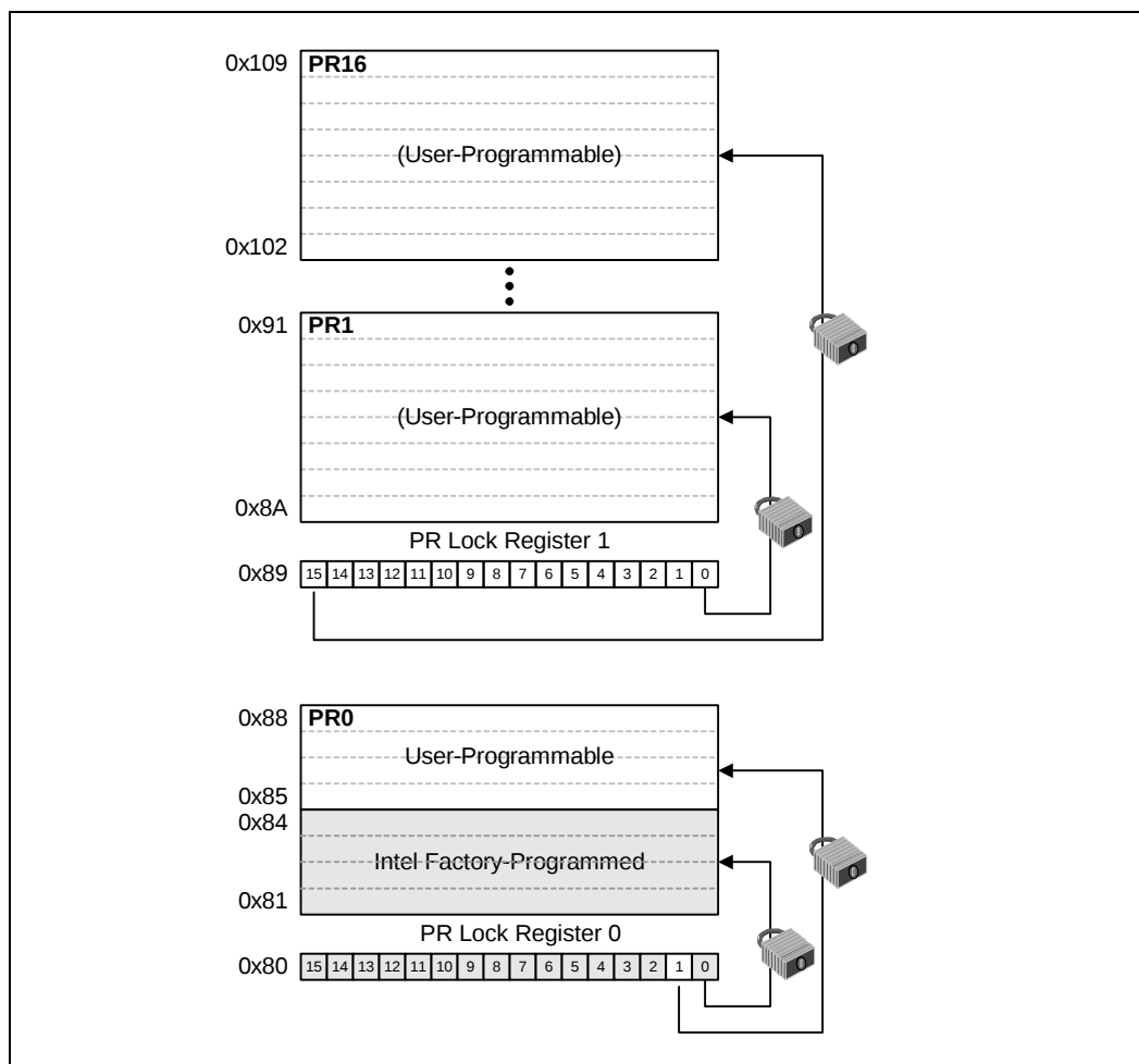
Figure 10. Protection Register Memory Map
