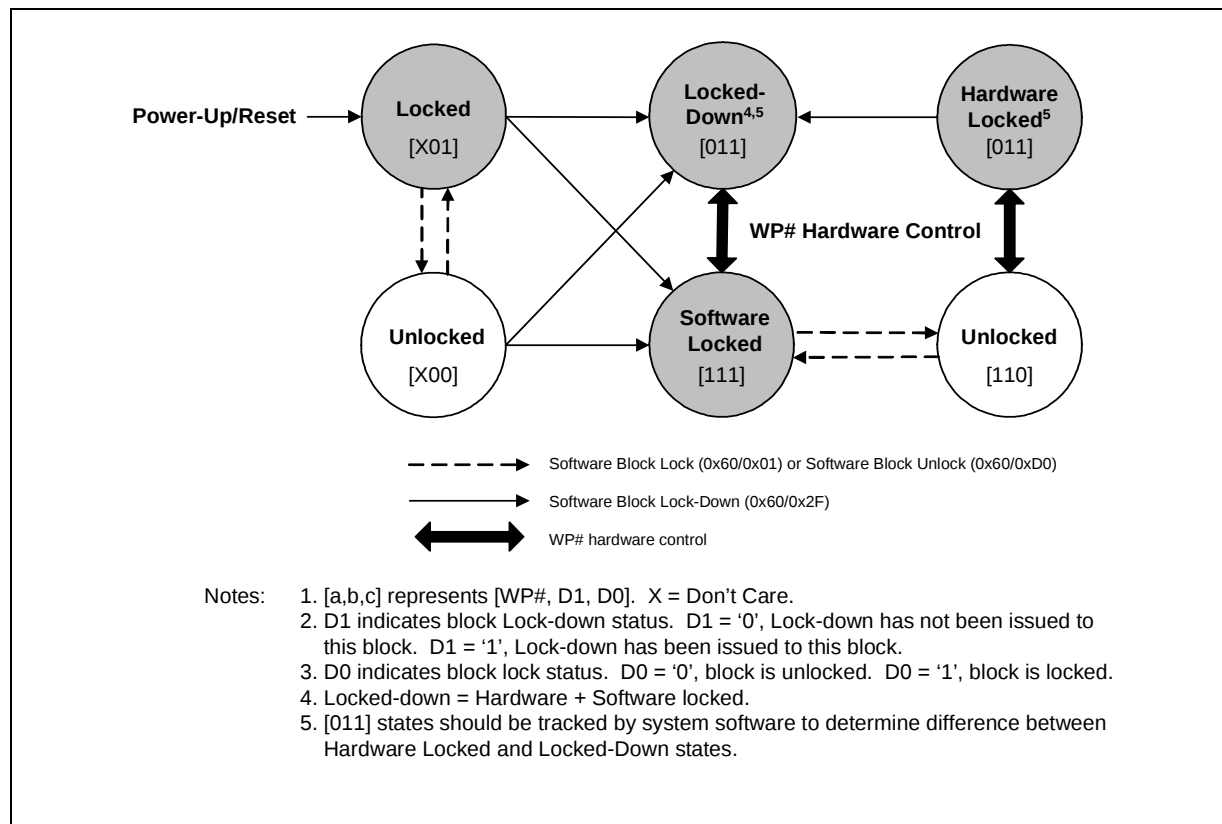
Figure 9. Block Locking State Diagram
