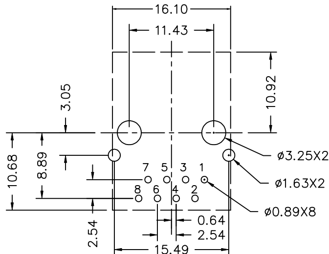
Recommended PCB layout (Component Side View)
