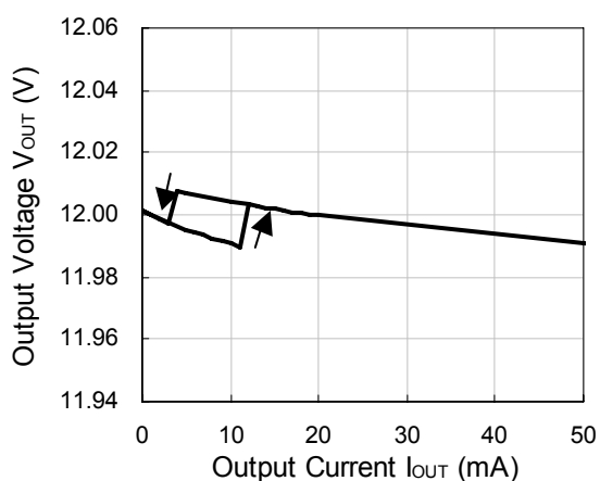
R1510S (VR=12.0V)
