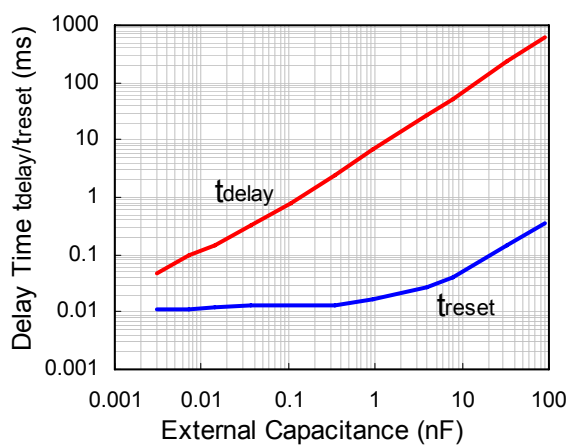
R1510SxxxC/D (VD=12.0V)
