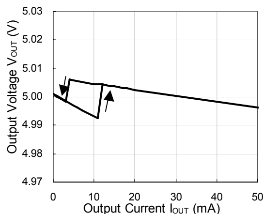
R1510S (VR=5.0V)
