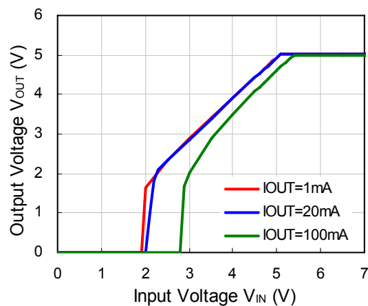
R1510S (VR=5.0V)
