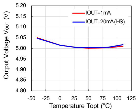
R1510S (VR=5.0V)
