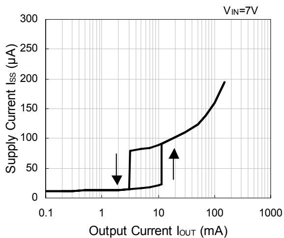
R1510SxxxA (VR=5.0V)
