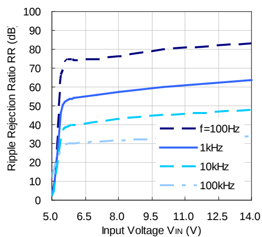
R1513S501B/D ( I_{OUT} = 50 \text{ mA} )
