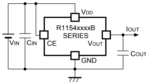
R1154xxxxxB Typical Application
