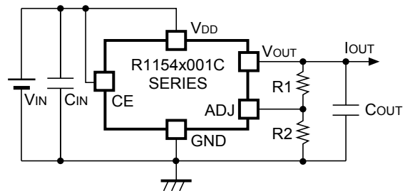
R1154xxxxxC Typical Application
