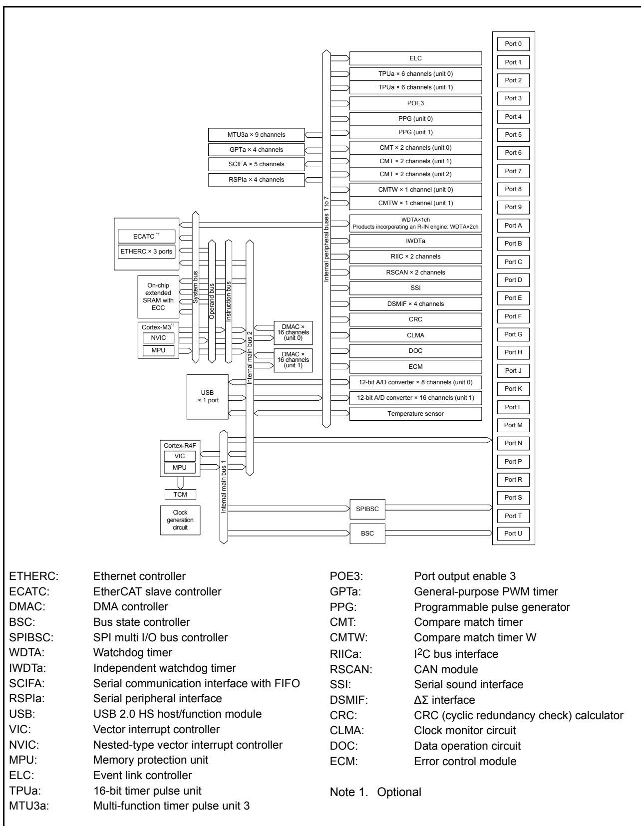
Figure 1.1 Block Diagram
