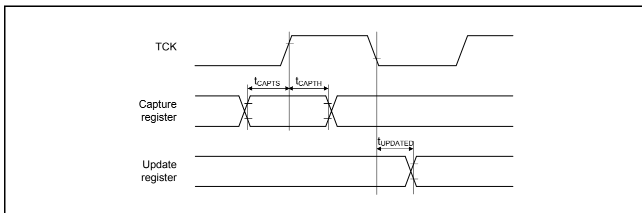
Figure 2.89 Boundary Scan Input/Output Timing
