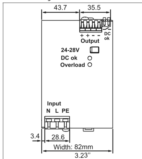
Fig. 20-1 Front view
