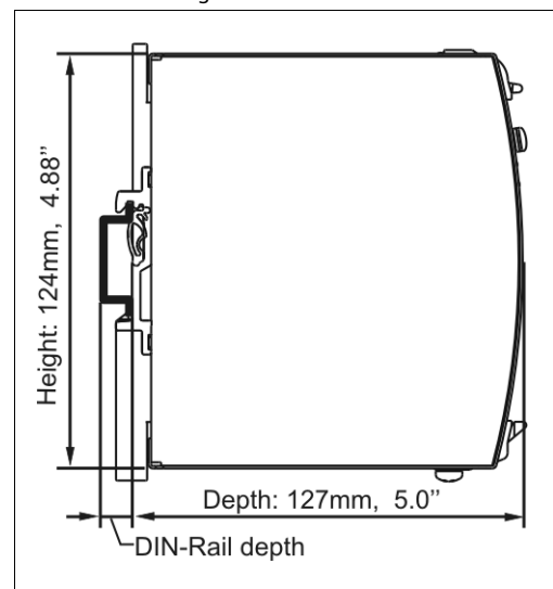
Fig. 20-2 Side view
