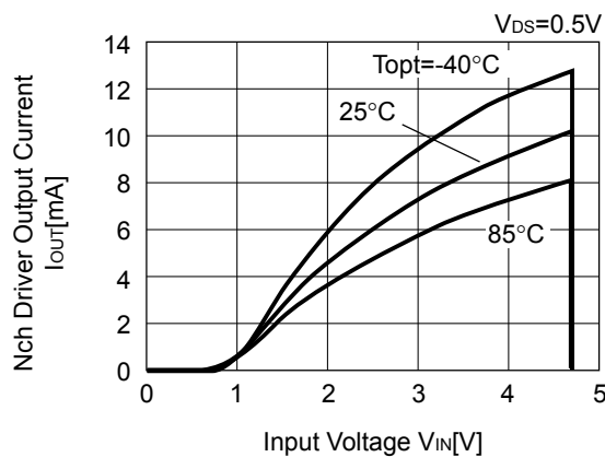
R3130N46xx5
