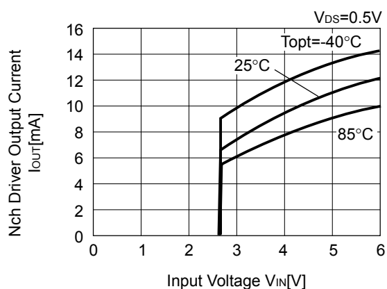
R3131N26xx3
