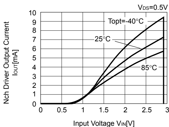
R3130N29xx3
