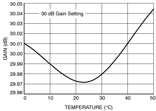
Figure 15. Gain vs. Temperature (30 dB)
