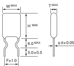
Cut / formed lead type.
