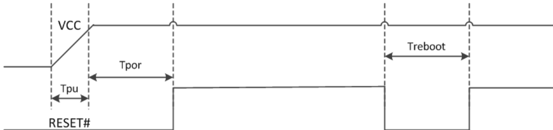
Figure 6 Reset Timing
