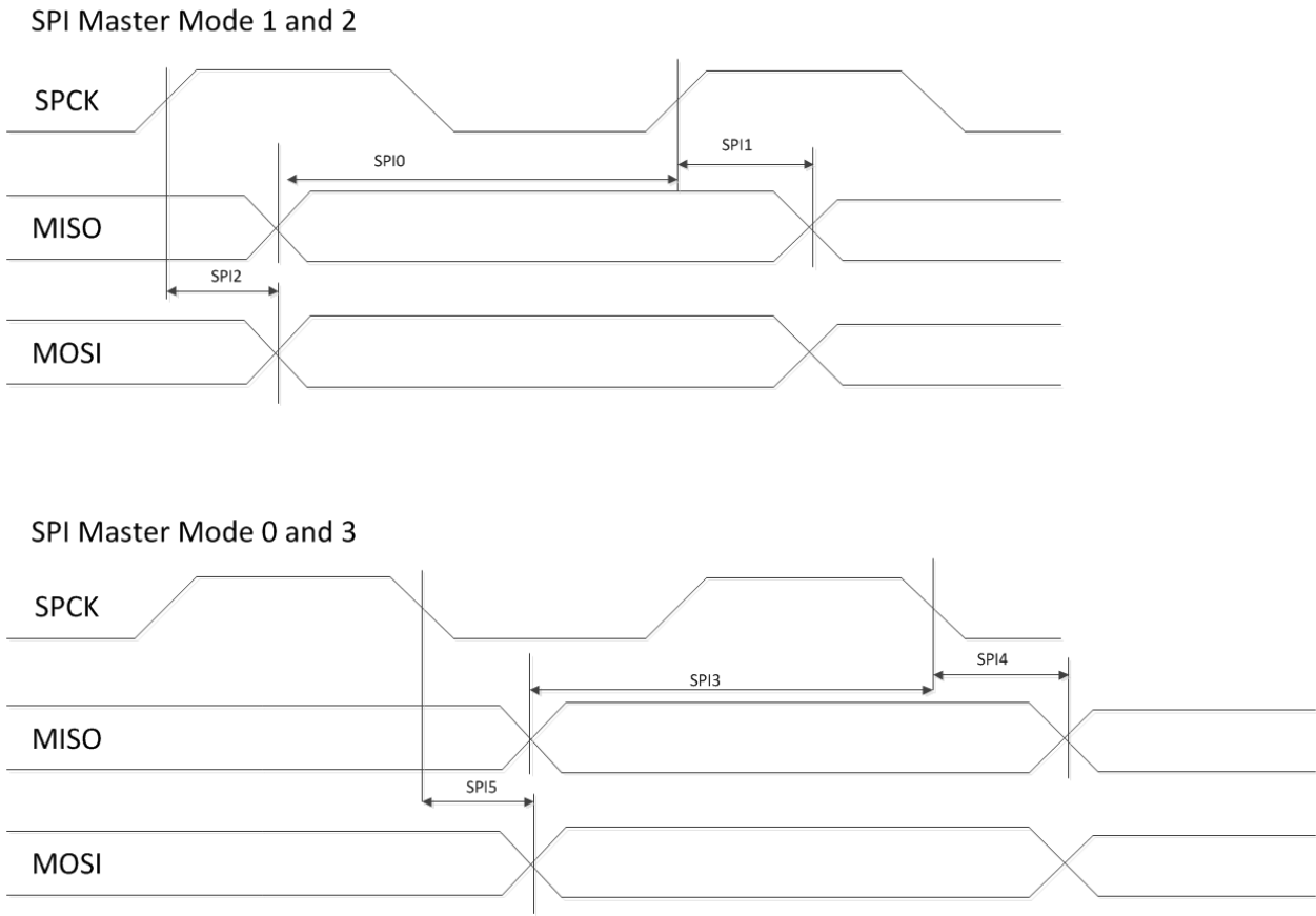
Figure 3 SPI Timing Diagram – Master Mode
