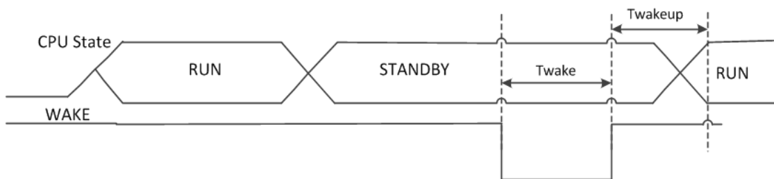
Figure 8 Wake Timing
