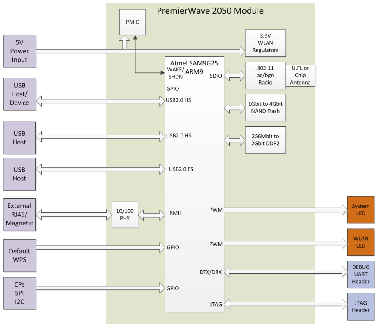
Figure 1 PremierWave 2050 Block Diagram
