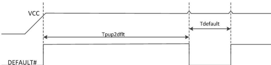
Figure 7 Reset to Defaults Timing
