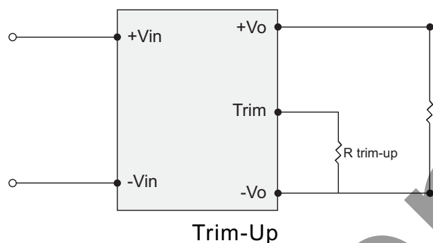
FIGURE 2: TRIM-UP VOLTAGE SETUP
