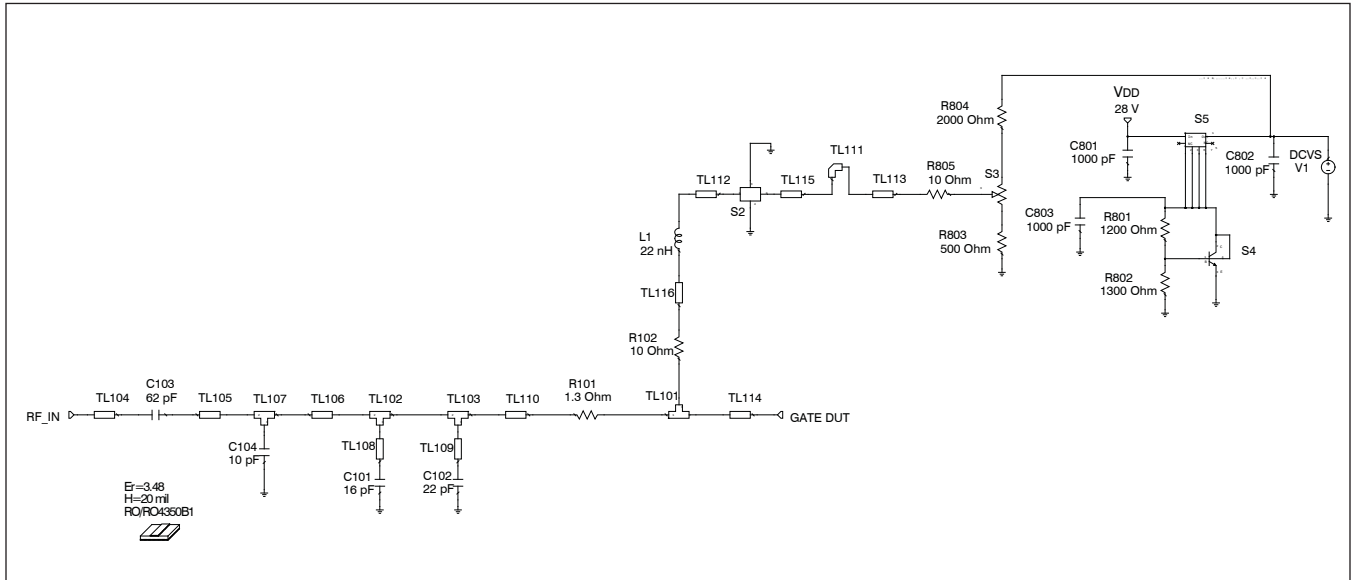
Reference circuit input schematic for f = 940 \text{ MHz}
