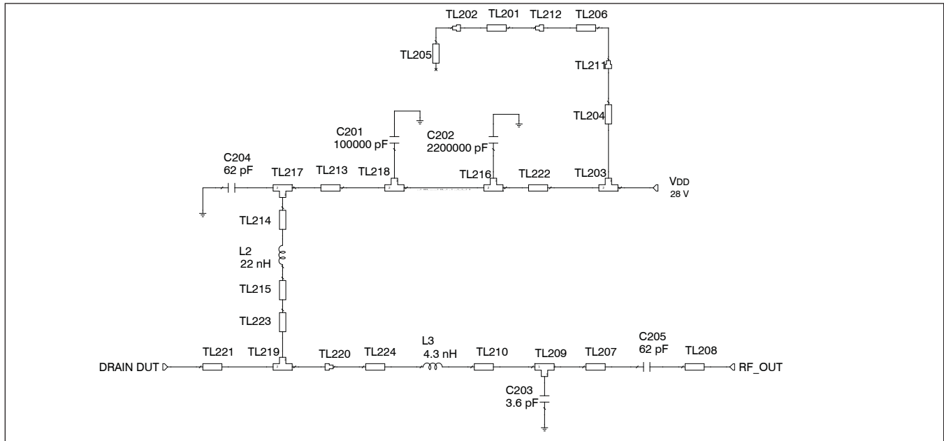
Reference circuit output schematic for f = 940 \text{ MHz}
