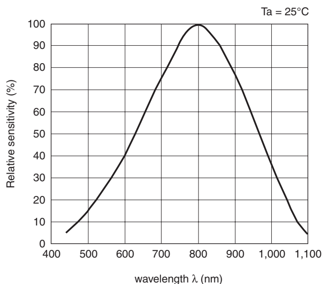
Fig. 2 Spectral Sensitivity
