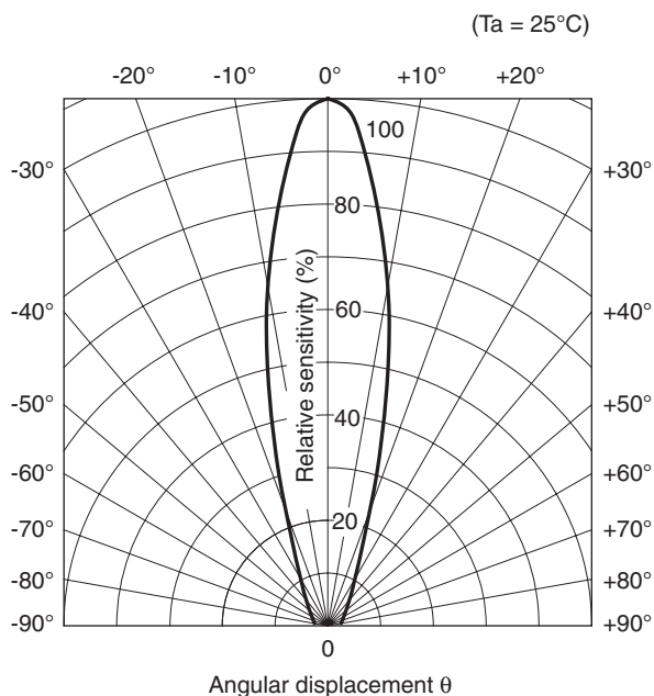
Fig. 3 Sensitivity Diagram
