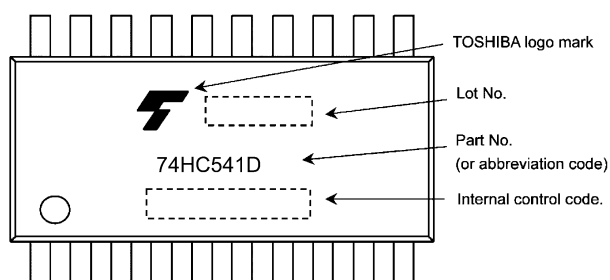
74HC541D
