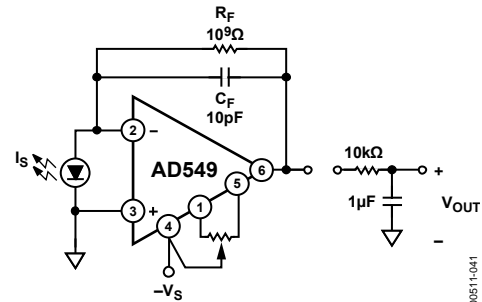
Figure 41. Photodiode Preamp
