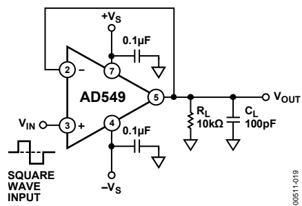
Figure 19. Unity-Gain Follower
