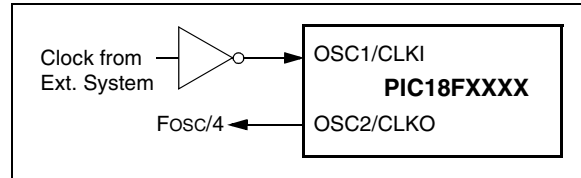
FIGURE 2-3: EXTERNAL CLOCK INPUT OPERATION (EC CONFIGURATION)
