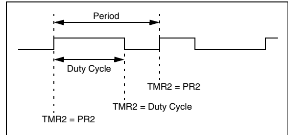
FIGURE 15-4: PWM OUTPUT
