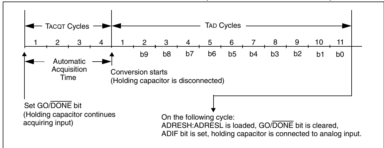
FIGURE 19-4: A/D CONVERSION TAD CYCLES ( \text{ACQT}<2:0> = 010 , \text{TACQ} = 4 \text{ TAD} )
