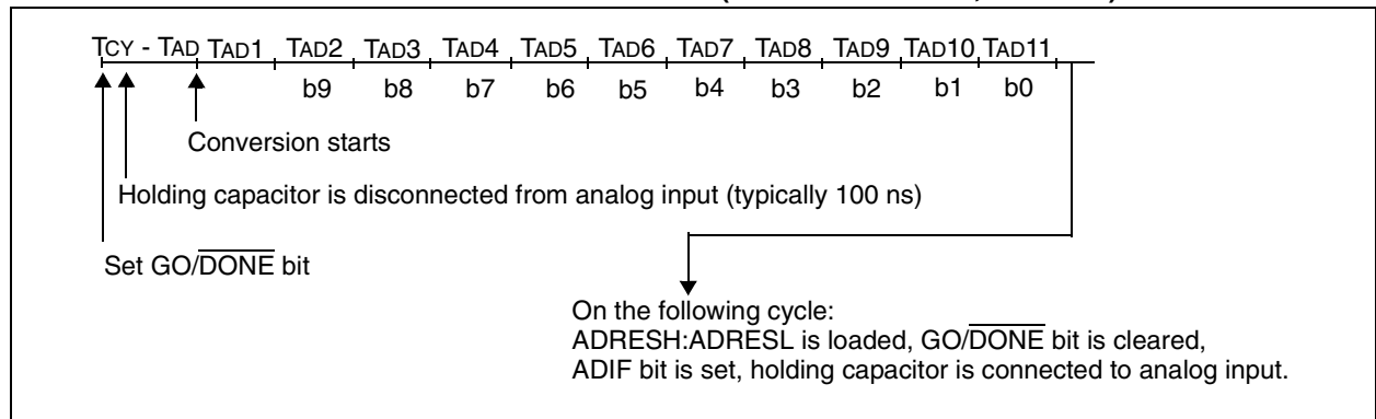
FIGURE 19-3: A/D CONVERSION TAD CYCLES ( \text{ACQT}<2:0> = 000 , \text{TACQ} = 0 )
