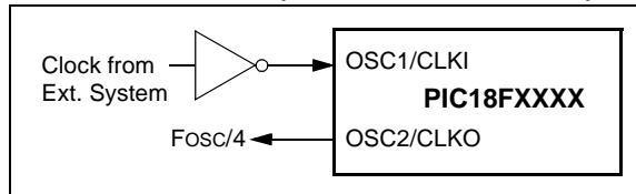
FIGURE 2-3: EXTERNAL CLOCK INPUT OPERATION (EC CONFIGURATION)
