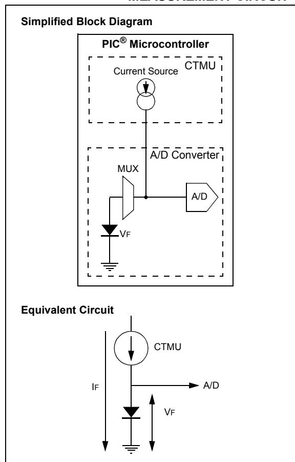
FIGURE 26-4: CTMU TEMPERATURE MEASUREMENT CIRCUIT
