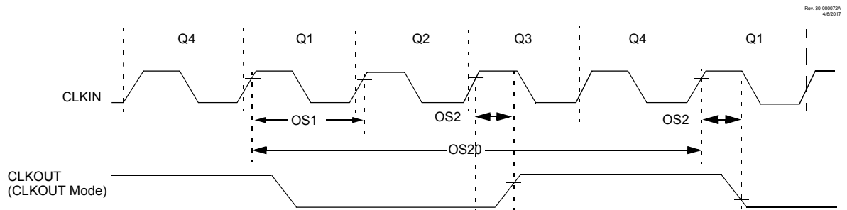
Figure 40-5. Clock Timing
