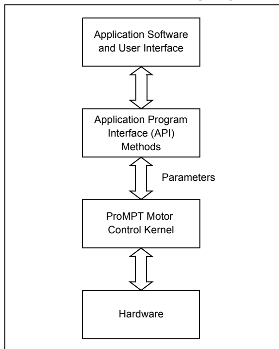
FIGURE 14-3: LAYERS OF THE MOTOR CONTROL ARCHITECTURE STACK
