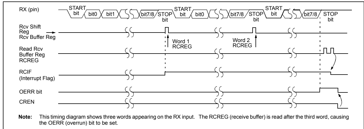
FIGURE 17-5: ASYNCHRONOUS RECEPTION
