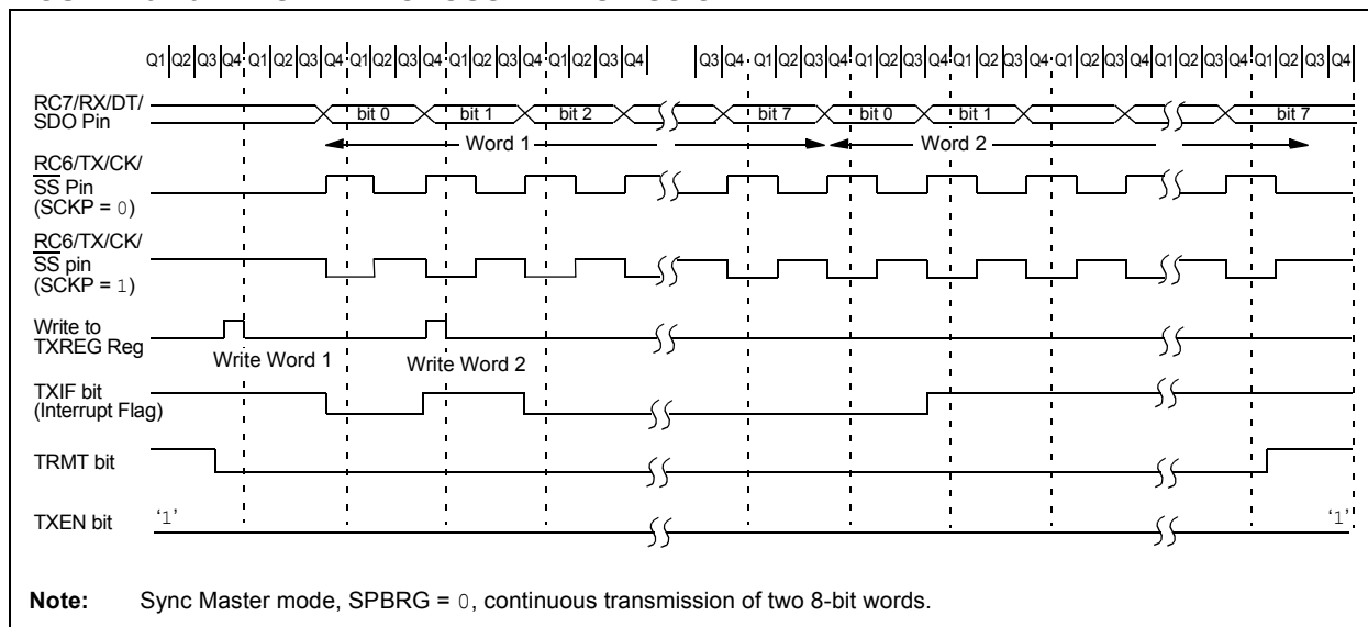
FIGURE 19-10: SYNCHRONOUS TRANSMISSION
