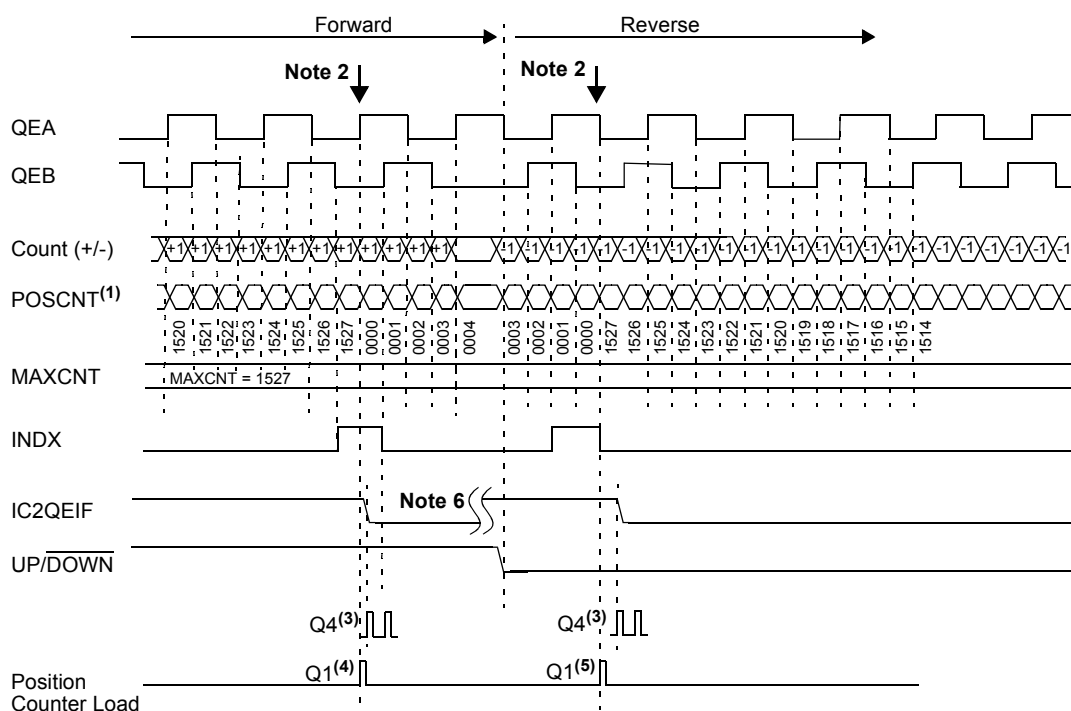
FIGURE 16-11: QE1 MODULE RESET TIMING WITH THE INDEX INPUT
