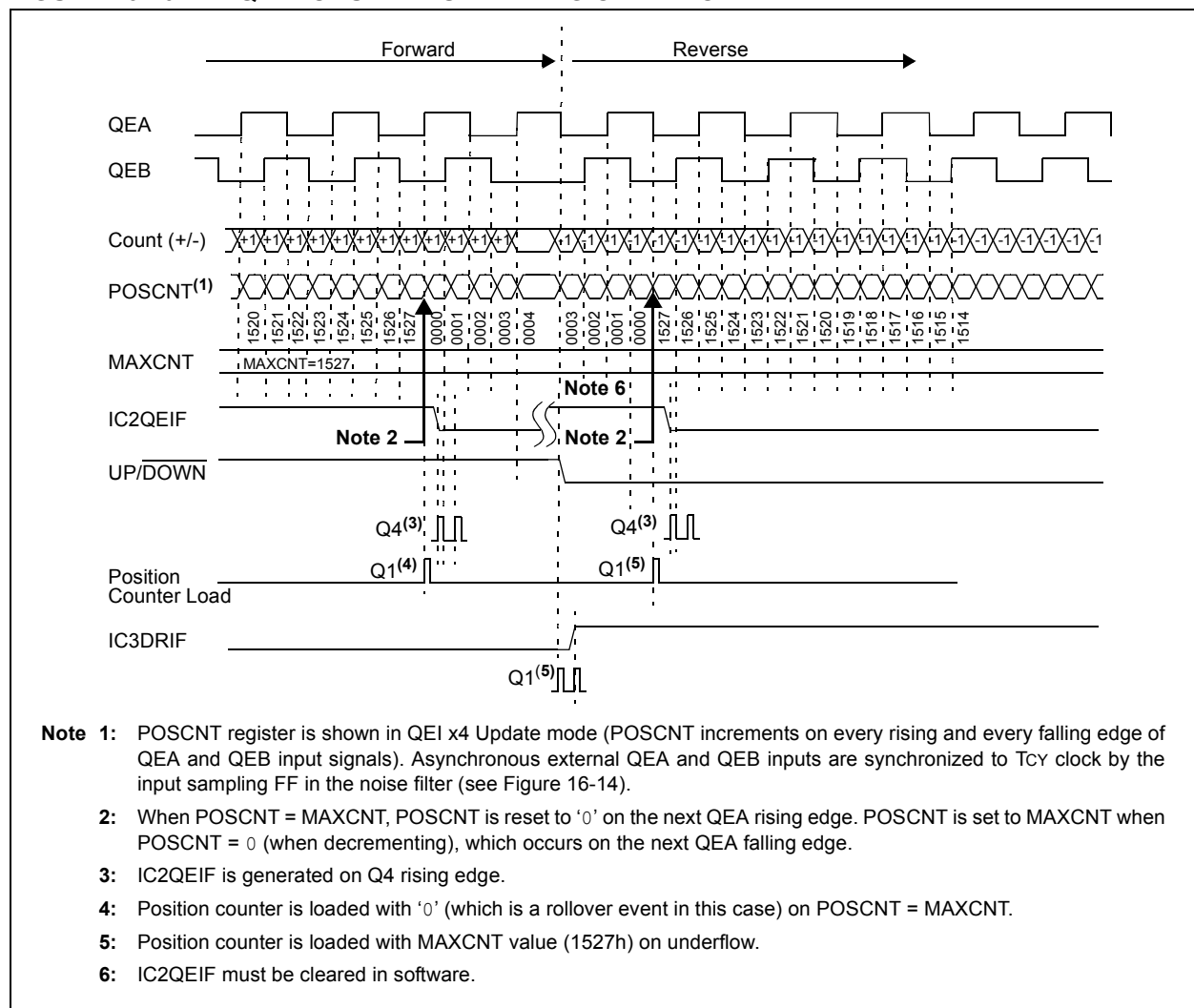
FIGURE 16-10: QE1 MODULE RESET TIMING ON PERIOD MATCH
