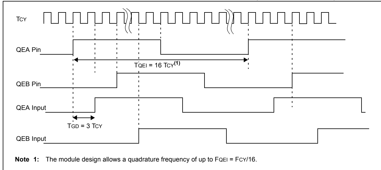
FIGURE 16-9: QE1 INPUTS WHEN SAMPLED BY THE FILTER (DIVIDE RATIO = 1:1)
