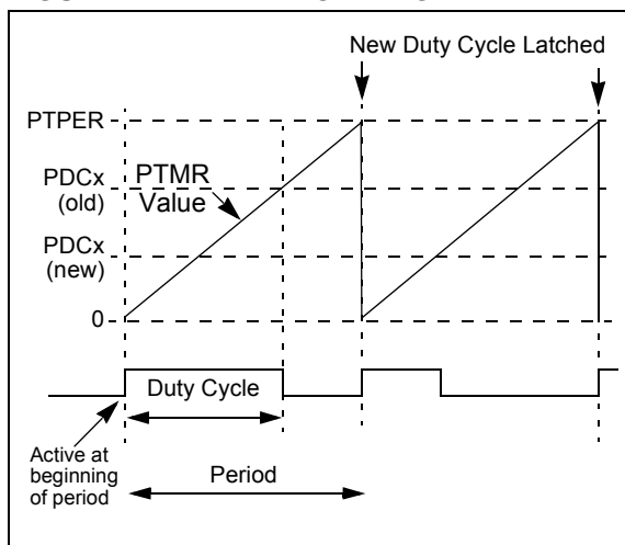
FIGURE 17-12: EDGE-ALIGNED PWM
