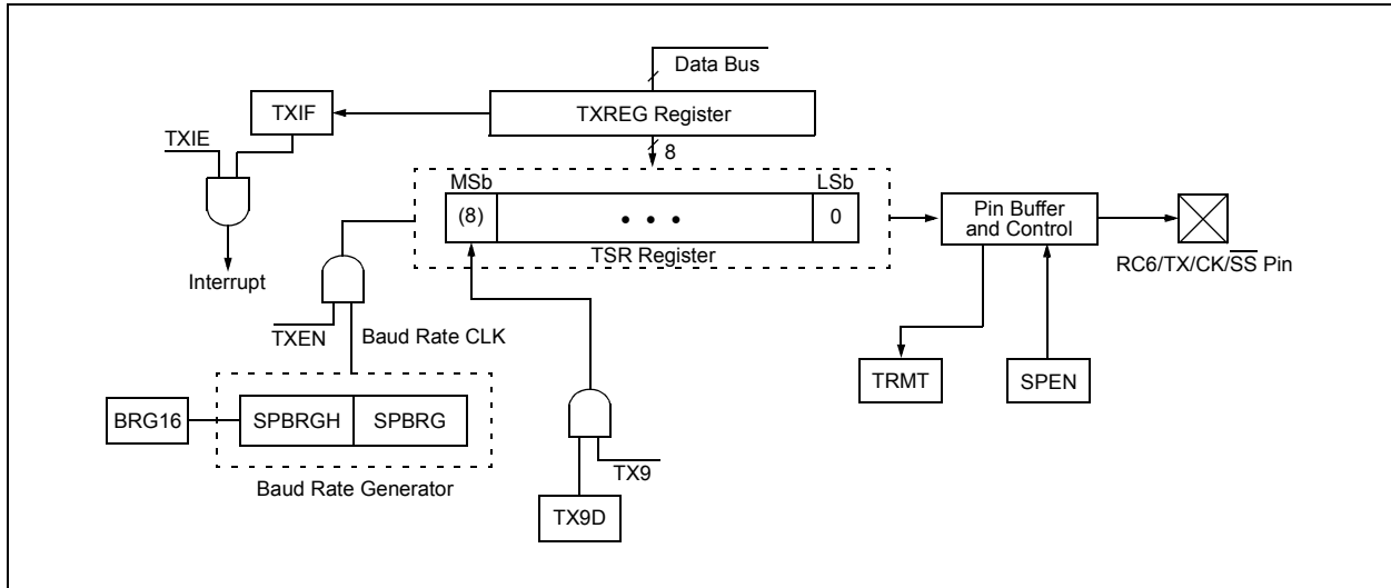
FIGURE 19-2: EUSART TRANSMIT BLOCK DIAGRAM
