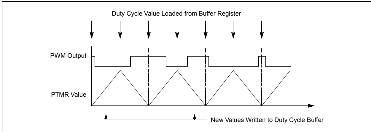
FIGURE 17-14: DUTY CYCLE UPDATE TIMES IN CONTINUOUS UP/DOWN COUNT MODE WITH DOUBLE UPDATES
