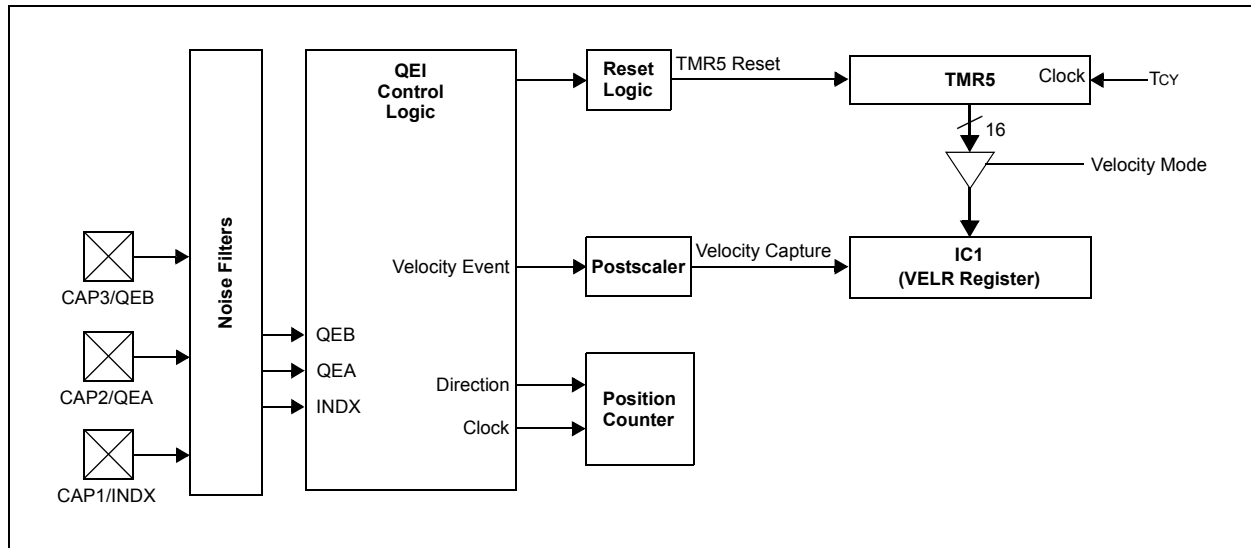
FIGURE 16-12: VELOCITY MEASUREMENT BLOCK DIAGRAM
