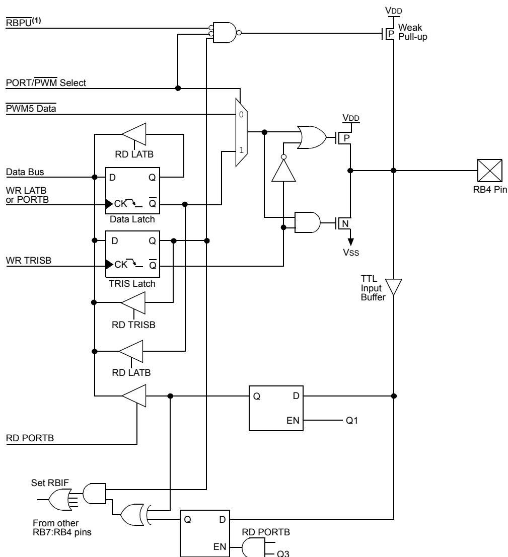
FIGURE 10-10: BLOCK DIAGRAM OF RB4
