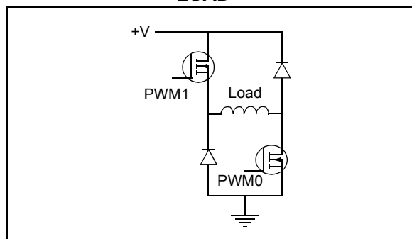
FIGURE 17-19: CENTER CONNECTED LOAD
