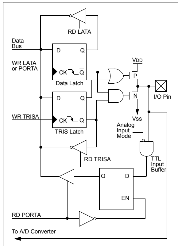
FIGURE 10-2: BLOCK DIAGRAM OF RA0
