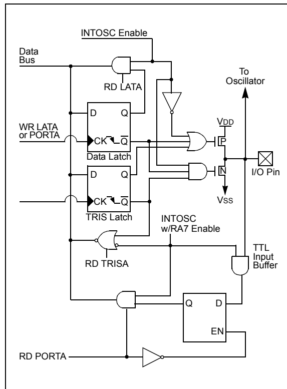
FIGURE 10-8: BLOCK DIAGRAM OF RA7
