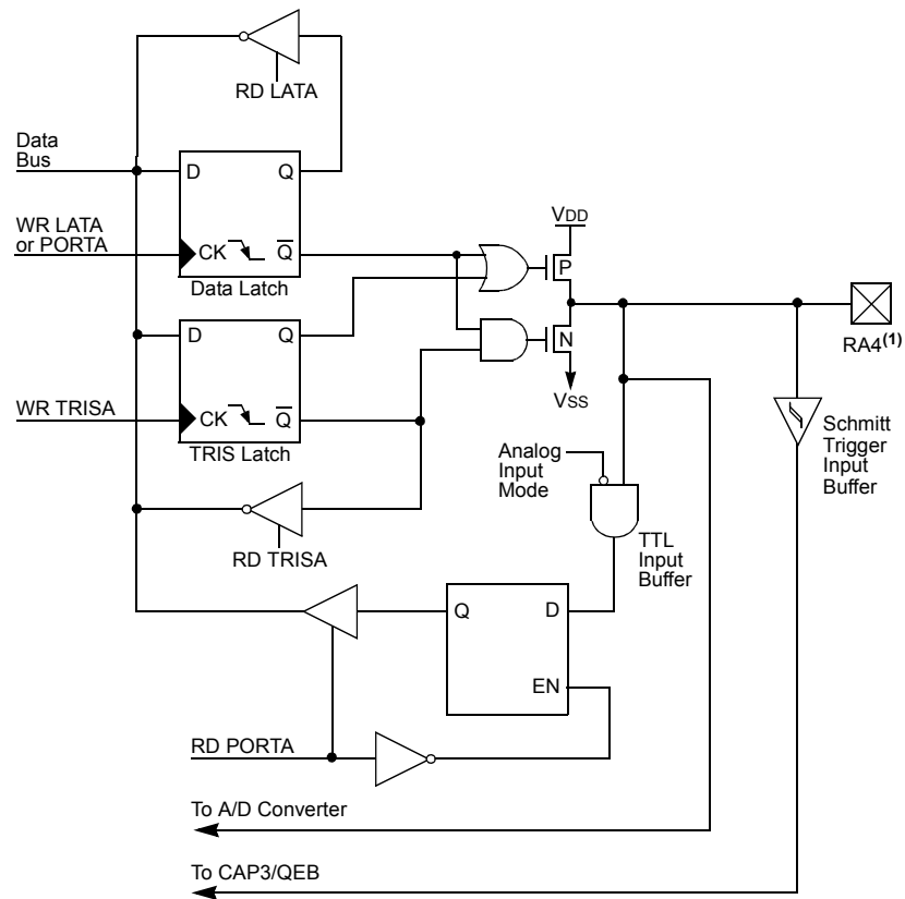
FIGURE 10-5: BLOCK DIAGRAM OF RA4
