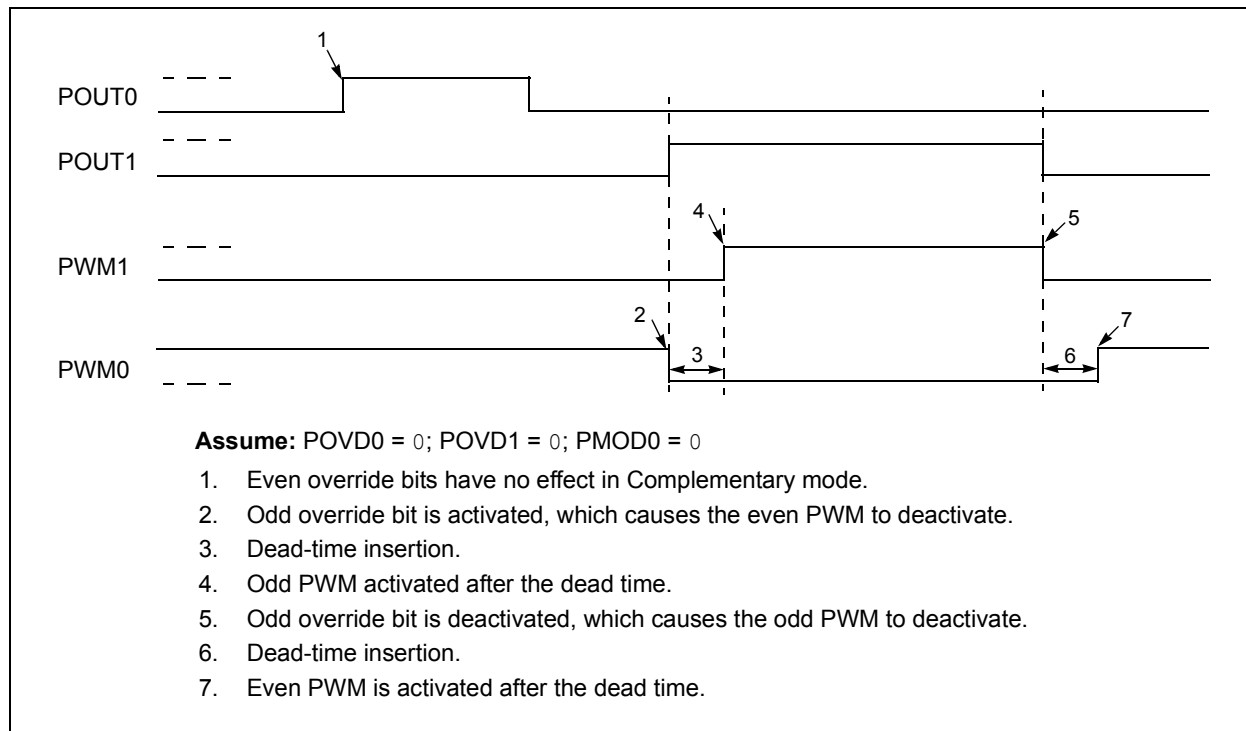
FIGURE 17-20: PWM OVERRIDE BITS IN COMPLEMENTARY MODE
