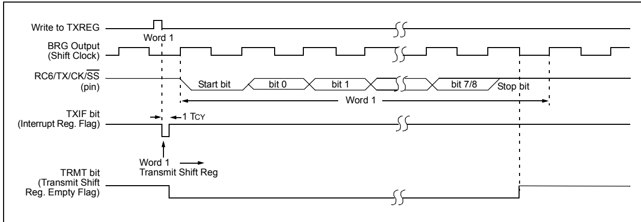
FIGURE 19-3: ASYNCHRONOUS TRANSMISSION
