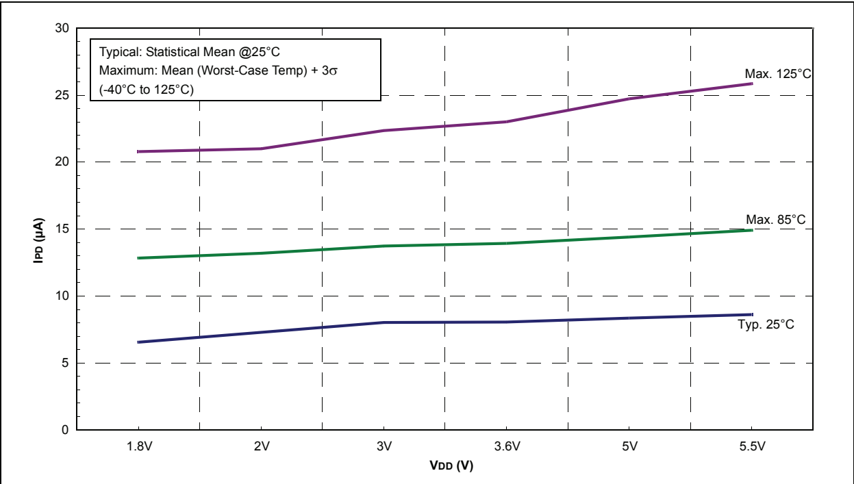
FIGURE 24-39: PIC16F722A/723A CAP SENSE LOW POWER I PD vs. V DD , V CAP = 0.1μF
