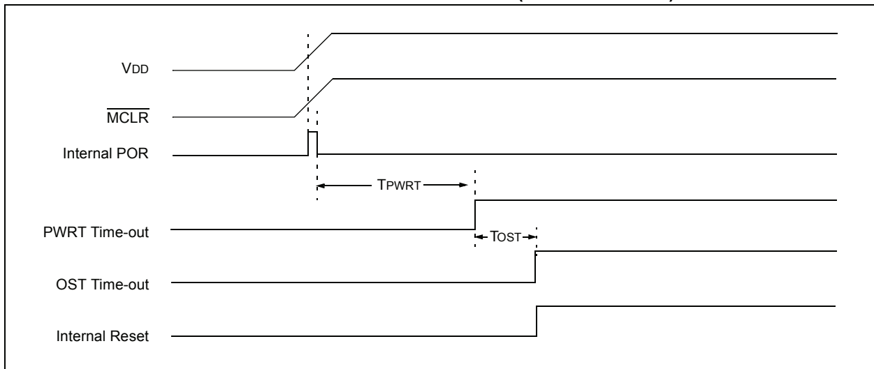
FIGURE 3-6: TIME-OUT SEQUENCE ON POWER-UP ( \overline{\text{MCLR}} WITH \text{VDD} ): CASE 3
