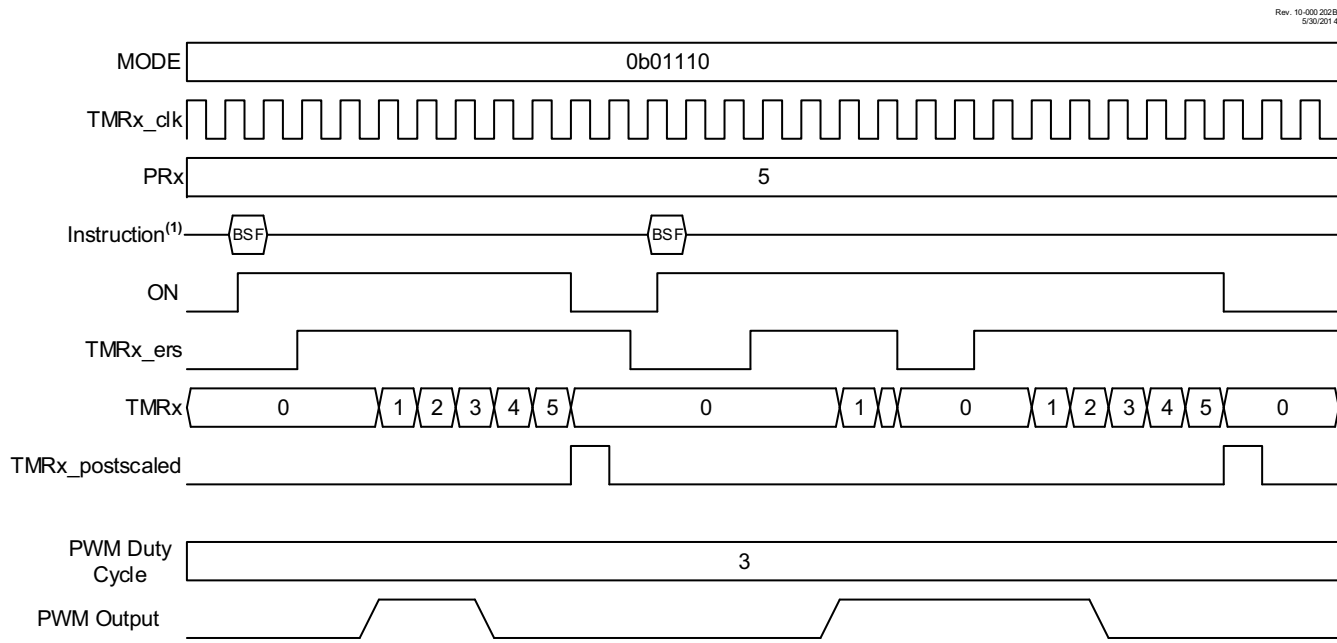
FIGURE 29-11: LOW LEVEL RESET, EDGE-TRIGGERED HARDWARE LIMIT ONE-SHOT MODE TIMING DIAGRAM (MODE = 01110)
