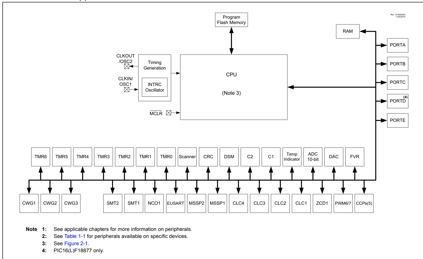
FIGURE 1-1: PIC16(L)F18857/77 BLOCK DIAGRAM
