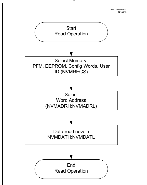
FIGURE 10-1: FLASH PROGRAM MEMORY READ FLOWCHART
