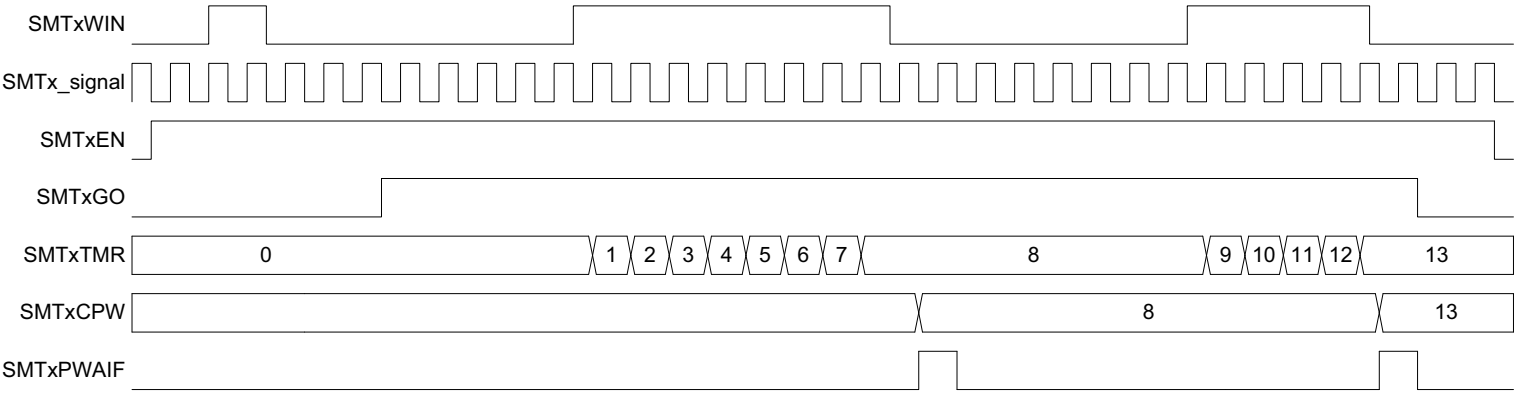
FIGURE 32-20: GATED COUNTER MODE SINGLE ACQUISITION TIMING DIAGRAM
