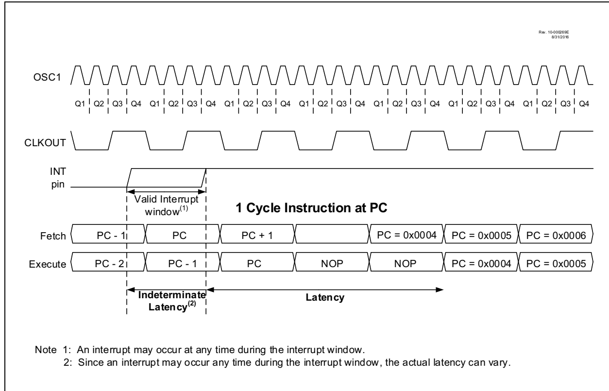
FIGURE 8-2: INTERRUPT LATENCY
