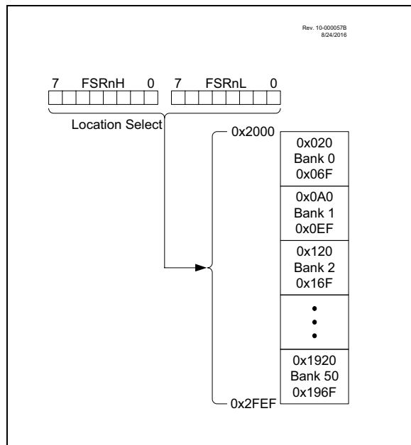
FIGURE 4-10: LINEAR DATA MEMORY MAP
