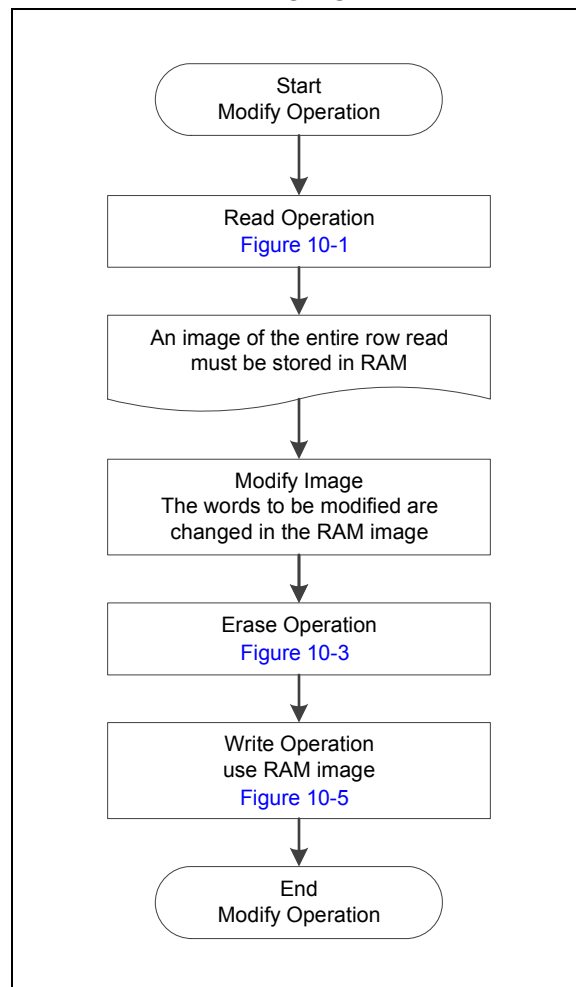
FIGURE 10-6: PROGRAM FLASH MEMORY MODIFY FLOWCHART
