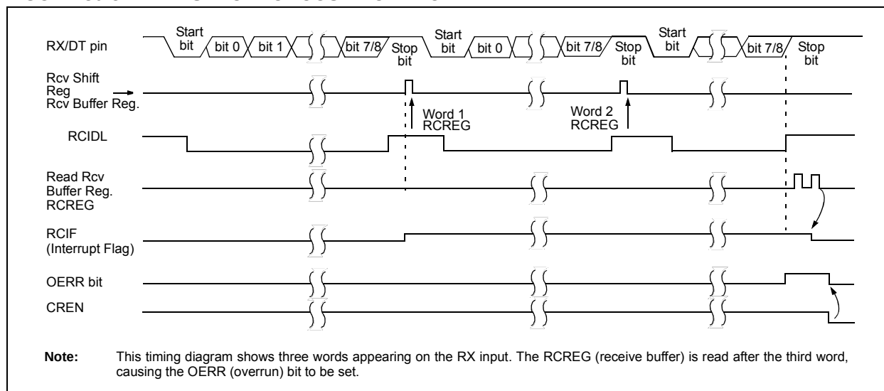
FIGURE 30-5: ASYNCHRONOUS RECEPTION
