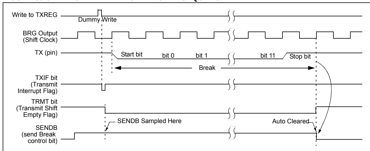
FIGURE 30-9: SEND BREAK CHARACTER SEQUENCE
