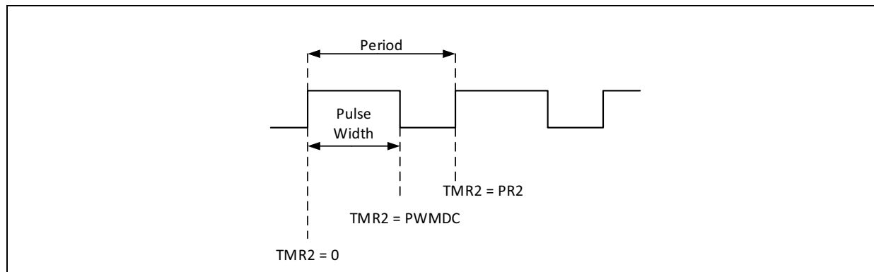
FIGURE 18-1: PWM OUTPUT
