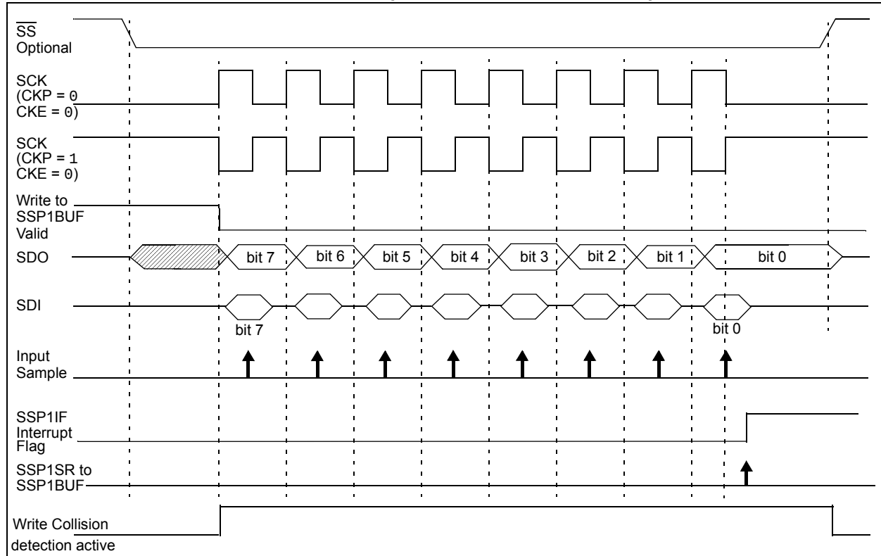
FIGURE 29-9: SPI MODE WAVEFORM (SLAVE MODE WITH CKE = 0)
