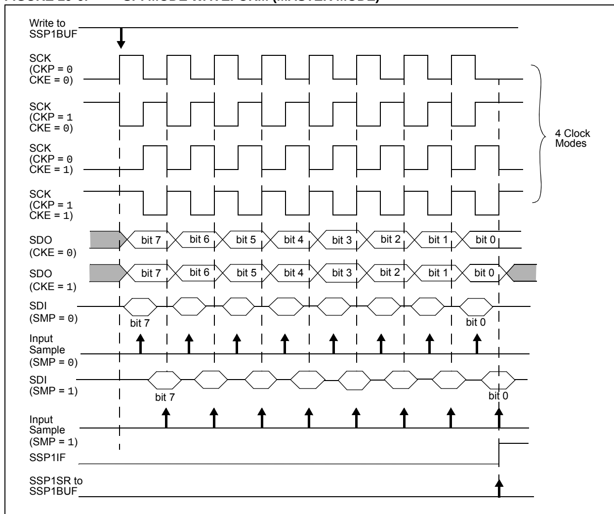
FIGURE 29-6: SPI MODE WAVEFORM (MASTER MODE)
