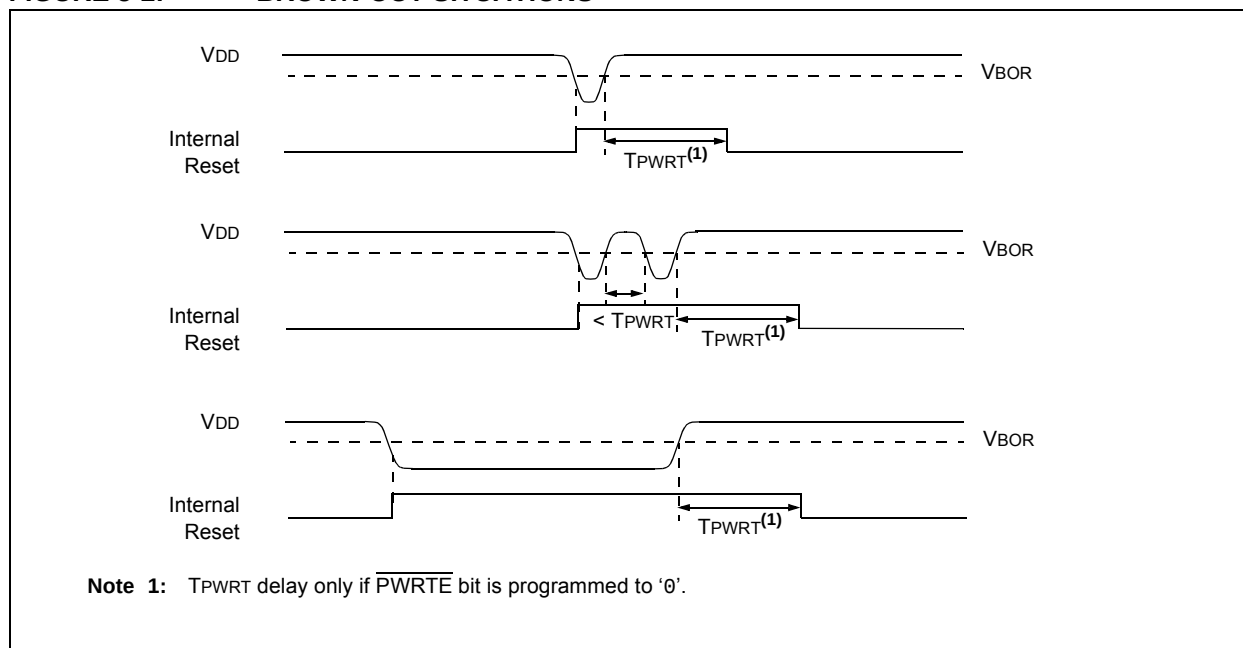
FIGURE 5-2: BROWN-OUT SITUATIONS
