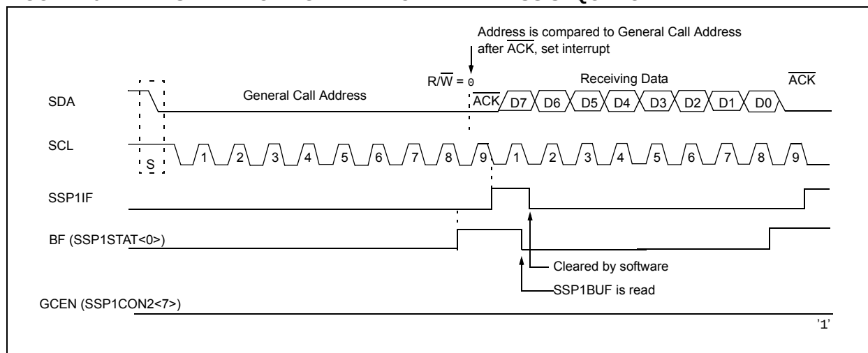
FIGURE 29-24: SLAVE MODE GENERAL CALL ADDRESS SEQUENCE
