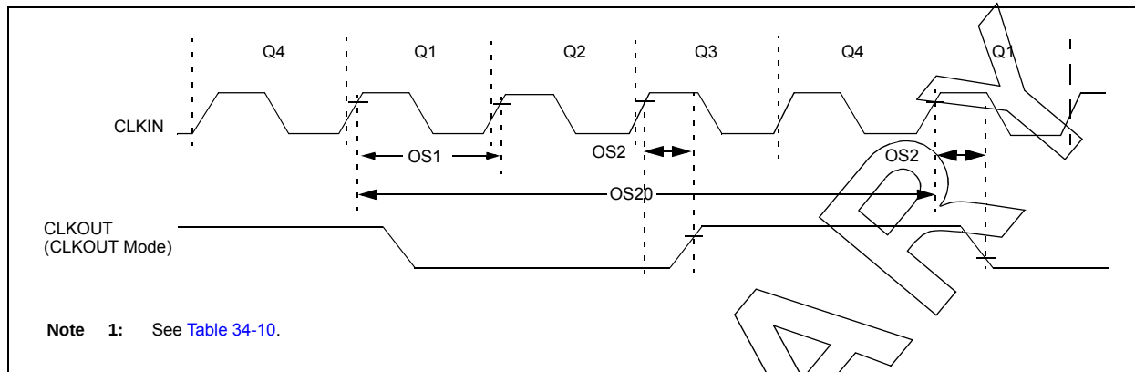
FIGURE 34-5: CLOCK TIMING
