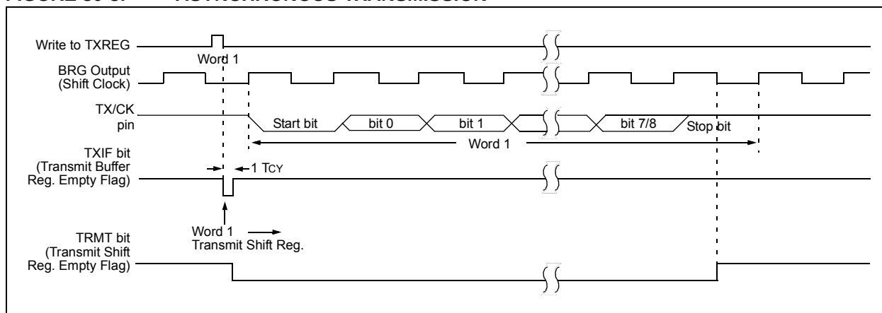
FIGURE 30-3: ASYNCHRONOUS TRANSMISSION
