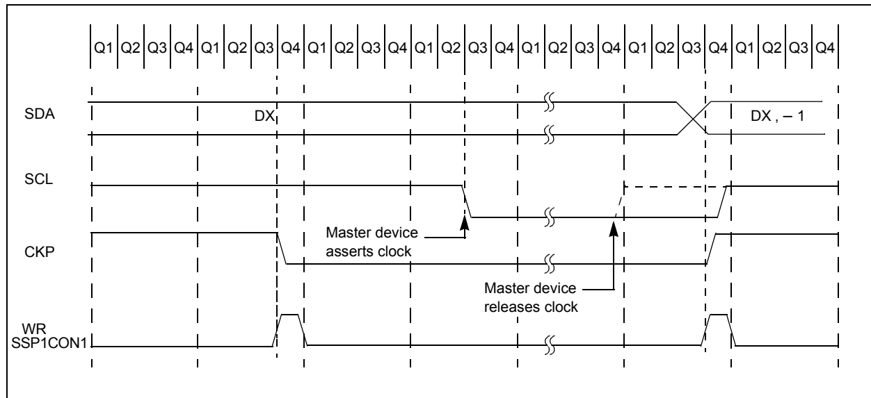
FIGURE 29-23: CLOCK SYNCHRONIZATION TIMING
