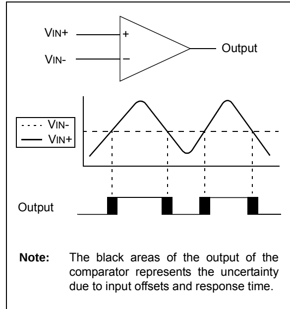
FIGURE 17-1: SINGLE COMPARATOR
