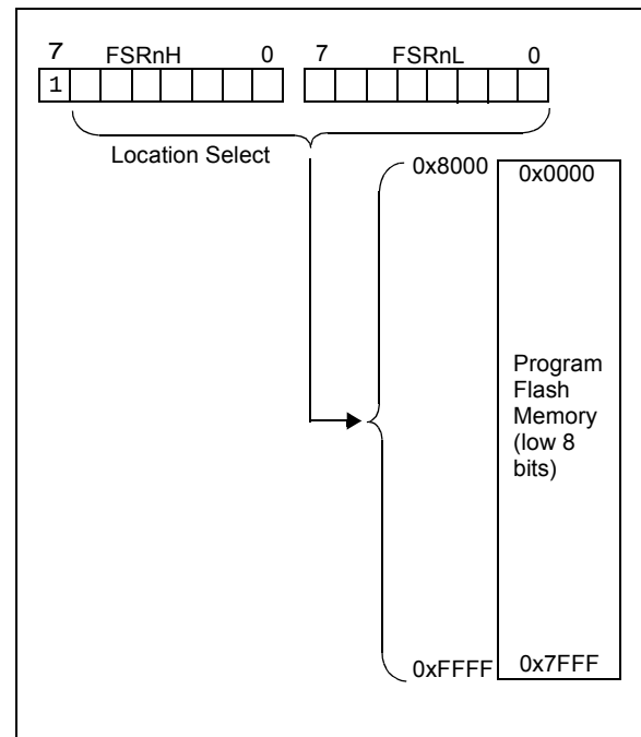
FIGURE 3-10: PROGRAM FLASH MEMORY MAP
