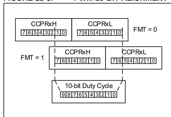
FIGURE 28-5: PWM 10-BIT ALIGNMENT
