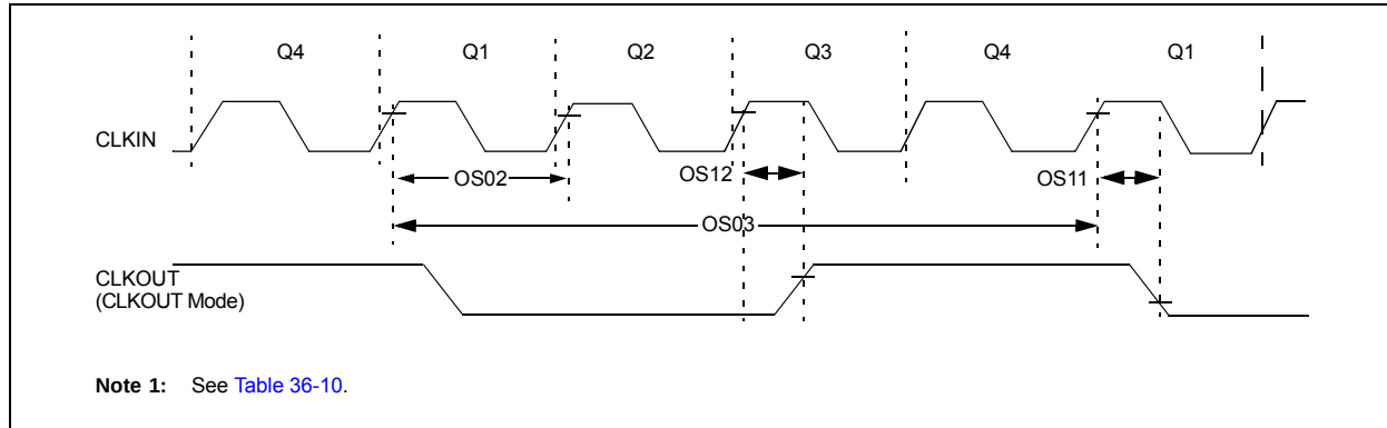
FIGURE 36-5: CLOCK TIMING
