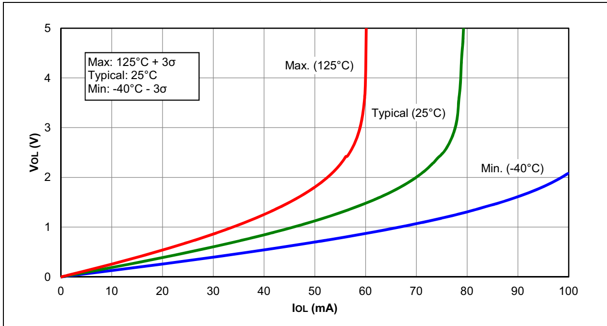
FIGURE 37-4: V_{OL} vs. I_{OL} OVER TEMPERATURE, V_{DD} = 3.0V
