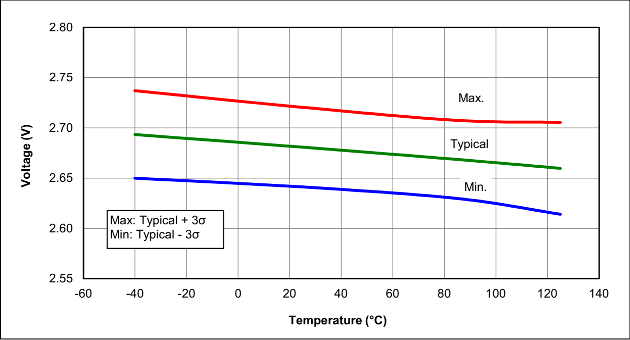
FIGURE 27-13: BROWN-OUT RESET VOLTAGE, BORV = 0
