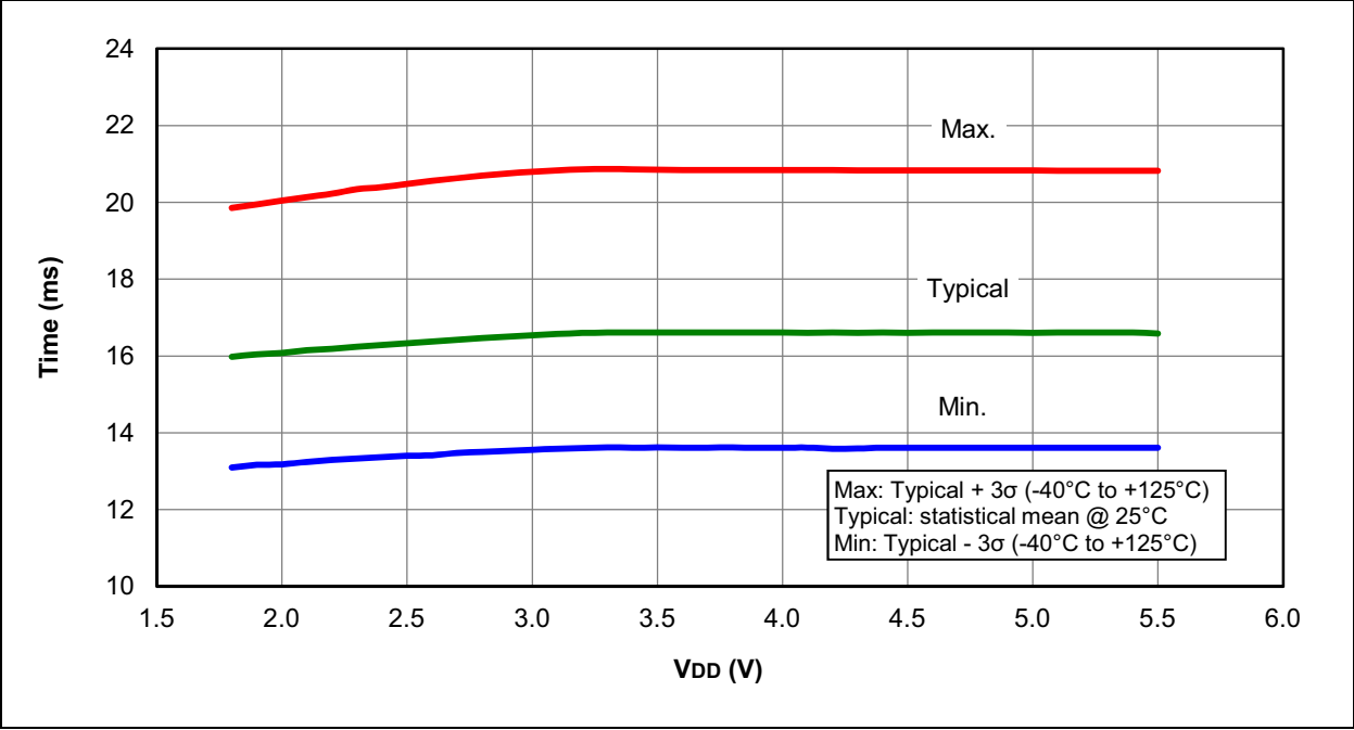
FIGURE 27-17: WDT TIME-OUT PERIOD
