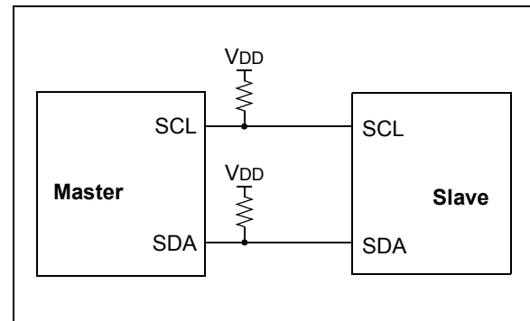
FIGURE 23-11: I 2 C MASTER/SLAVE CONNECTION
