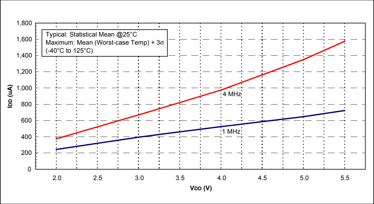
FIGURE 20-7: TYPICAL I_{DD} vs. V_{DD} OVER F_{osc} (EXTRC MODE)
