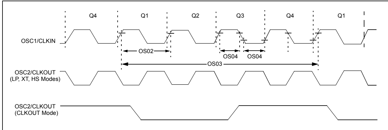
FIGURE 19-4: CLOCK TIMING
