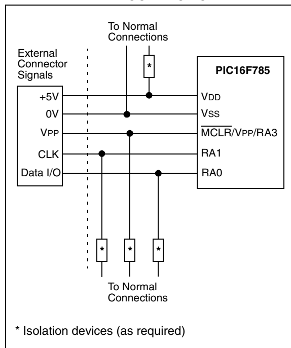
FIGURE 15-11: TYPICAL IN-CIRCUIT SERIAL PROGRAMMING CONNECTION
