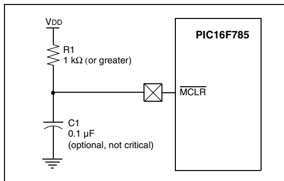
FIGURE 15-2: RECOMMENDED \overline{MCLR} CIRCUIT
