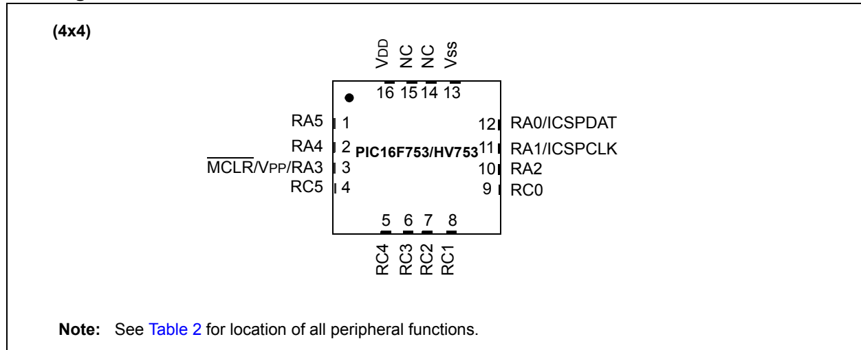
Pin Diagram – 16-Pin QFN
