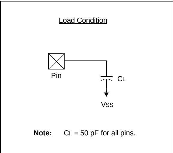
FIGURE 22-3: LOAD CONDITIONS
