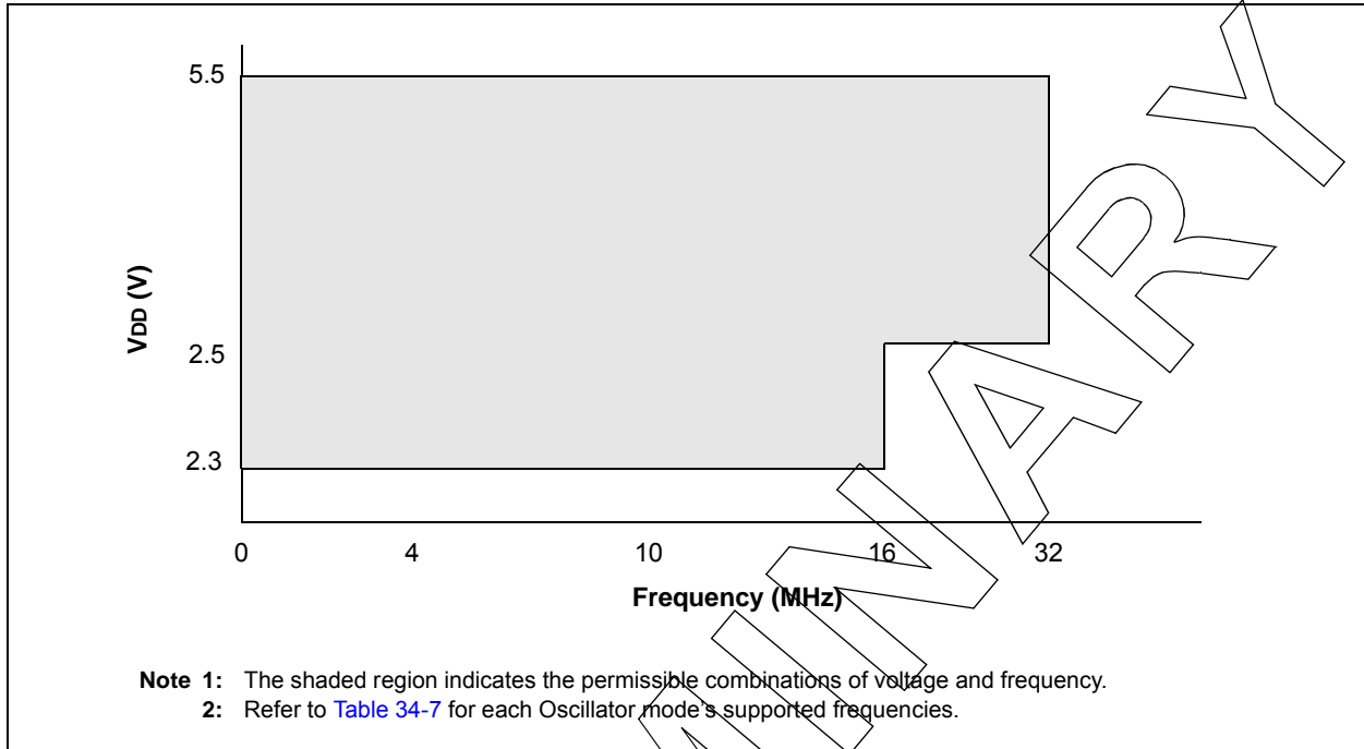
FIGURE 34-1: VOLTAGE FREQUENCY GRAPH, -40^{\circ}\text{C} \leq T_A \leq +125^{\circ}\text{C} , PIC16F18324/18344 ONLY
