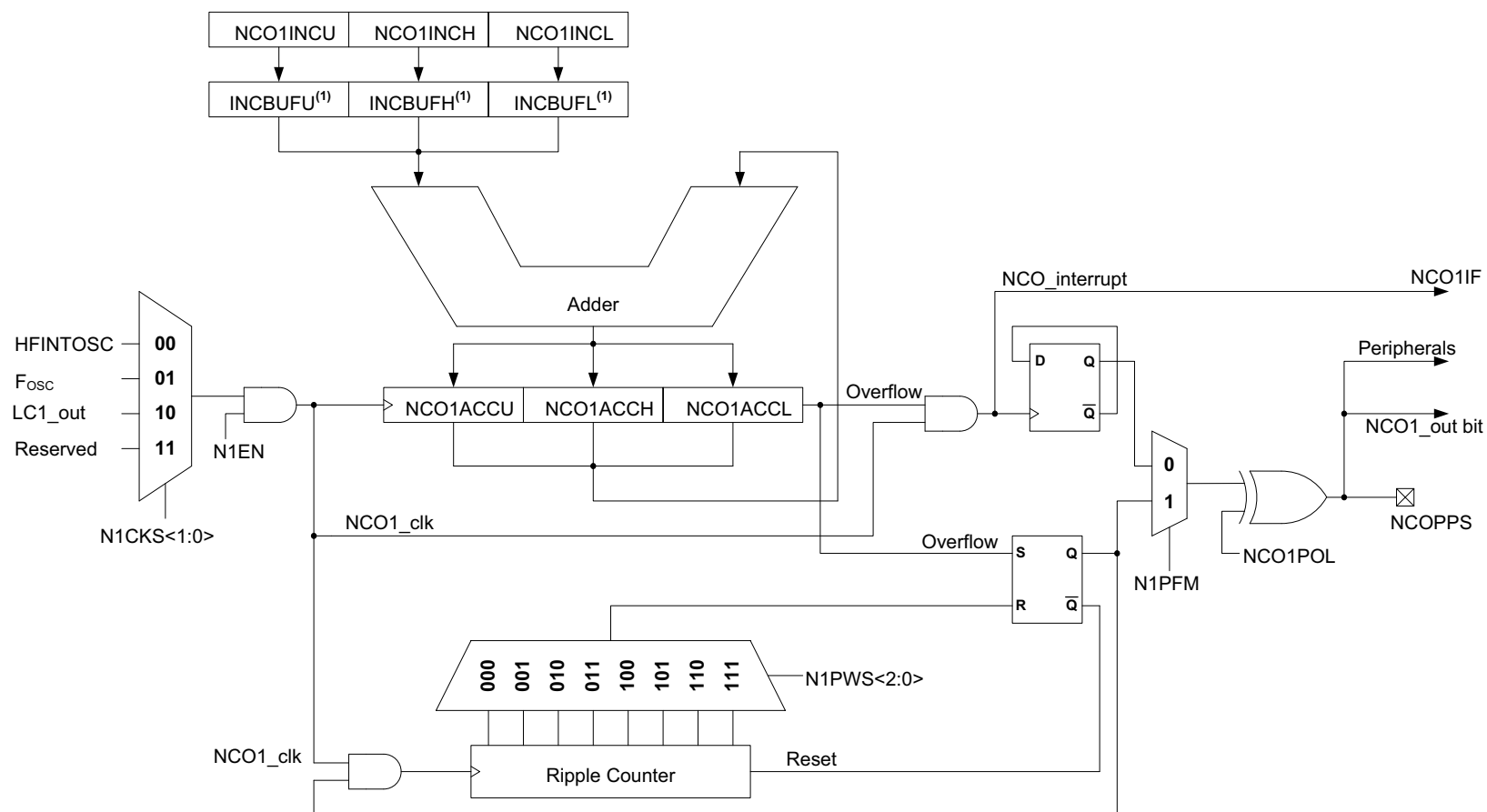
FIGURE 22-1: NUMERICALLY CONTROLLED OSCILLATOR MODULE SIMPLIFIED BLOCK DIAGRAM
