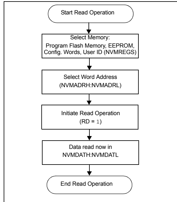
FIGURE 10-1: FLASH PROGRAM MEMORY READ FLOWCHART
