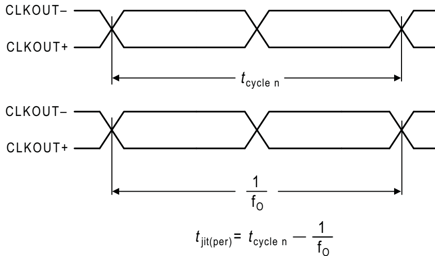
Figure 7. Period Jitter
