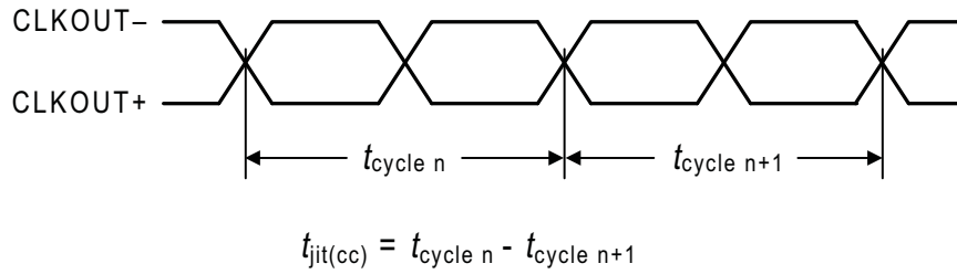
Figure 6. Cycle-to-Cycle Jitter
