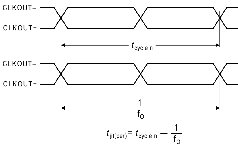
Figure 7. Period Jitter
