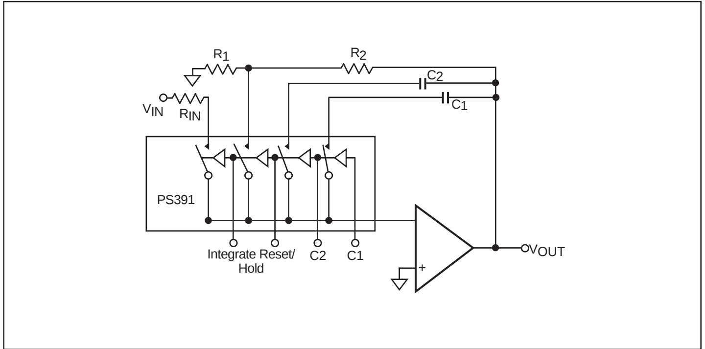
Figure 1. Programmable Integrator and Sample/Hold
