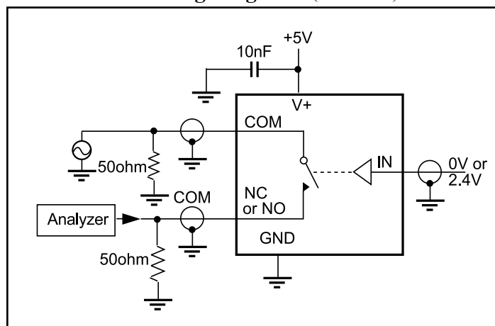
Figure 3. Off Isolation
