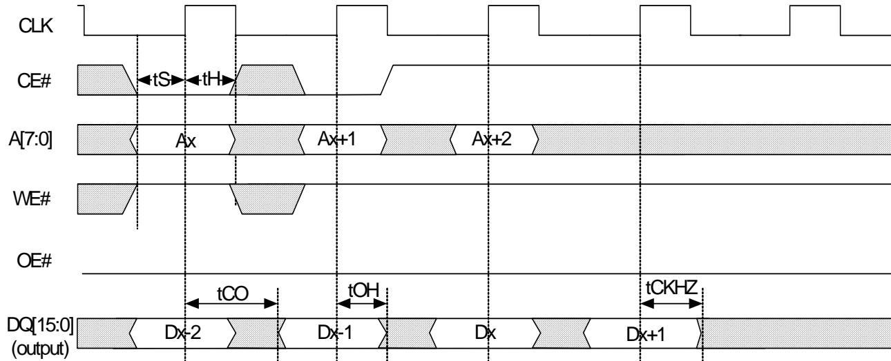
Figure 13. Synchronous Read (OE# Fixed LOW) Timing
