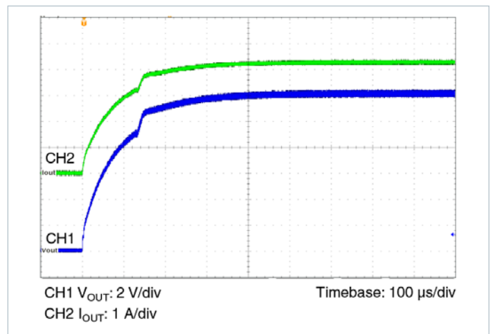
Figure 25 — Start Up, C_{REF} = 0 ( V_{IN} = 16\text{ V} , I_{OUT} = 4.2\text{ A} , C_R , C_{OUT} = 6 \times 2.2\text{ }\mu\text{F X7R Ceramic} )
