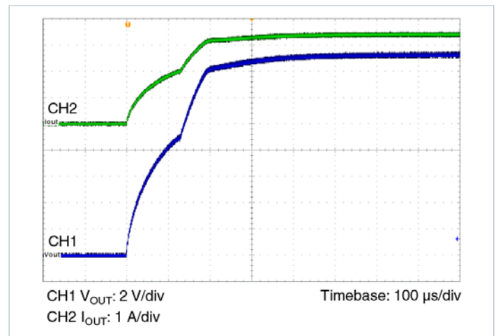
Figure 35 — Start Up, C_{REF} = 0 ( V_{IN} = 16\text{ V} , I_{OUT} = 3.3\text{ A} , C_R , C_{OUT} = 6 \times 2.2\text{ }\mu\text{F X7R Ceramic} )
