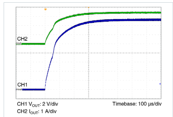
Figure 36 — Start Up, C_{REF} = 0 ( V_{IN} = 28\text{ V} , I_{OUT} = 3.3\text{ A} , C_R , C_{OUT} = 6 \times 2.2\text{ }\mu\text{F X7R Ceramic} )
