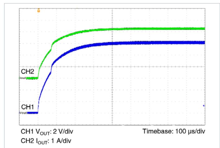
Figure 26 — Start Up, C_{REF} = 0 ( V_{IN} = 28\text{ V} , I_{OUT} = 4.2\text{ A} , C_R , C_{OUT} = 6 \times 2.2\text{ }\mu\text{F X7R Ceramic} )
