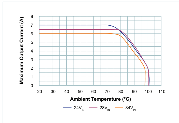
Figure 21 — Thermal de-rating @ V_{OUT} = 30V with Limited Input Range
