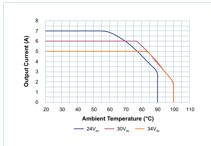
Figure 22 — Thermal de-rating @ V_{OUT} = 34V with Limited Input Range
