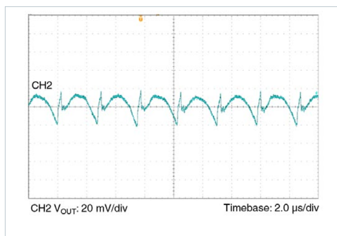
Figure 5 — Output Ripple 12 V IN 1.0 V OUT at 15 A; C_{OUT} = 8 x 100 \mu F
