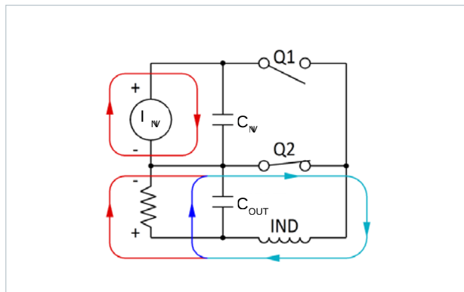
Figure 43 — Current flow: Q2 closed
