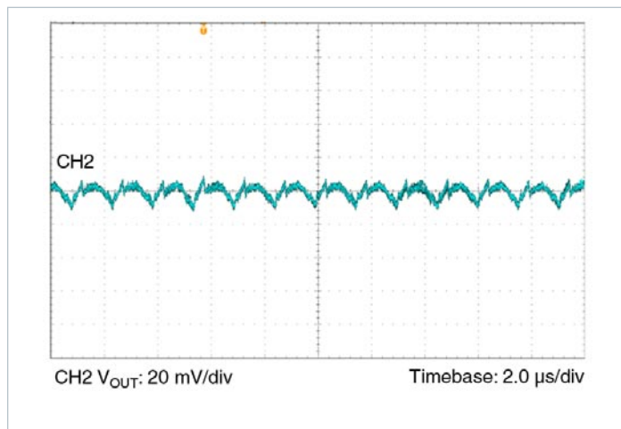
Figure 24 — Output Ripple 12 V_{IN} 3.3 V_{OUT} at 7.0 A; C_{OUT} = 8 x 100 \mu F
