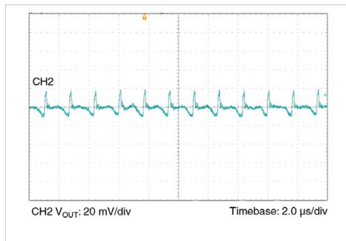
Figure 6 — Output Ripple 12 V IN 1.0 V OUT at 7.0 A; C_{OUT} = 8 x 100 \mu F
