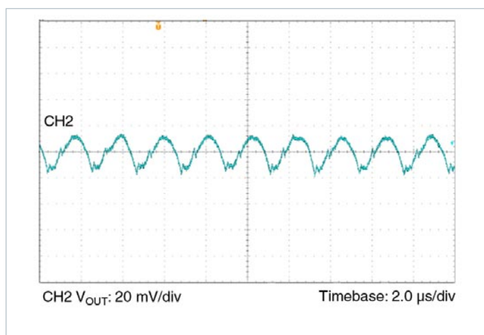
Figure 23 — Output Ripple 12 V_{IN} 3.3 V_{OUT} at 15 A; C_{OUT} = 8 x 100 \mu F
