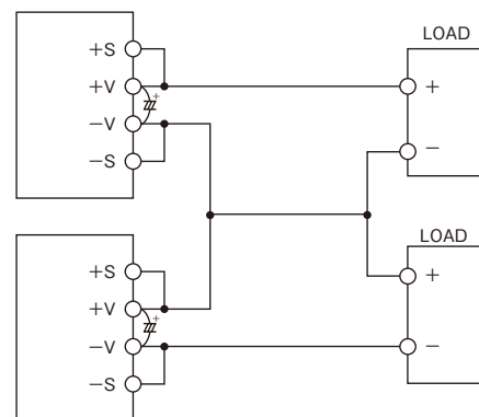
Figure 12-2: Series Operation using \pm Output
