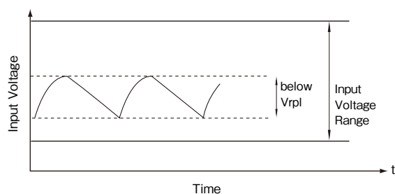
Figure1-1 Ripple Voltage
