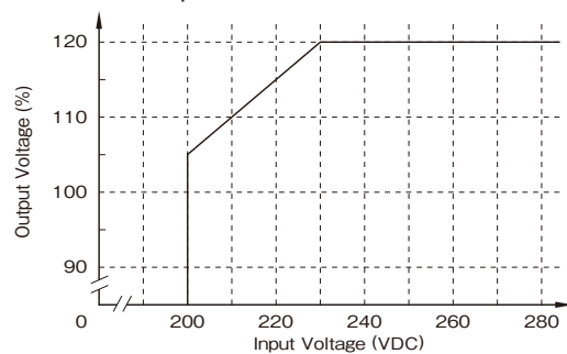
Figure2-5: Limitation of Input Voltage
