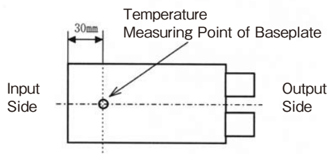
Figure 14-2 Temperature Measurement Point of Baseplate
