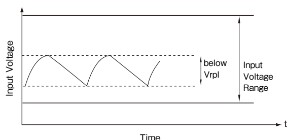
Figure1-1 Ripple Voltage
