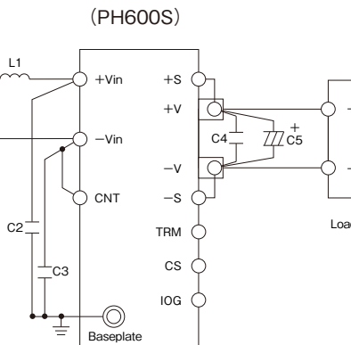
Figure1-2 Basic Connection
