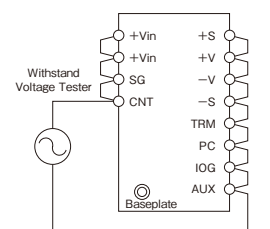
3kVAC for 1 minute (20mA) (24VDC Input model: 2kVAC)
