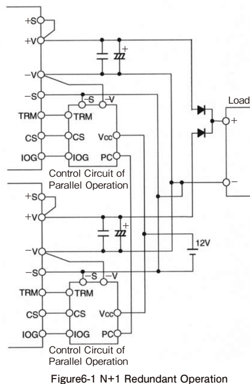
Figure6-1 N+1 Redundant Operation
