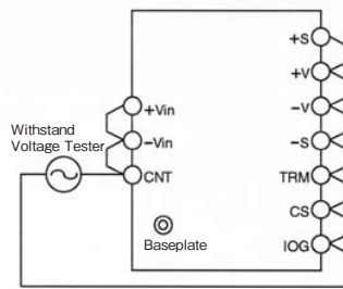
3kVAC 1 minute (20mA) (48VDC Input Model: 1.5kVAC) Figure20-2 Withstand Voltage Test for Input - Baseplate
