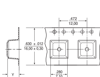
TAPE & REEL LAYOUT
